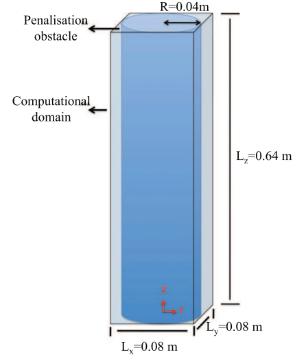
Fig. 2. Geometry and dimensions of the computational domain.
