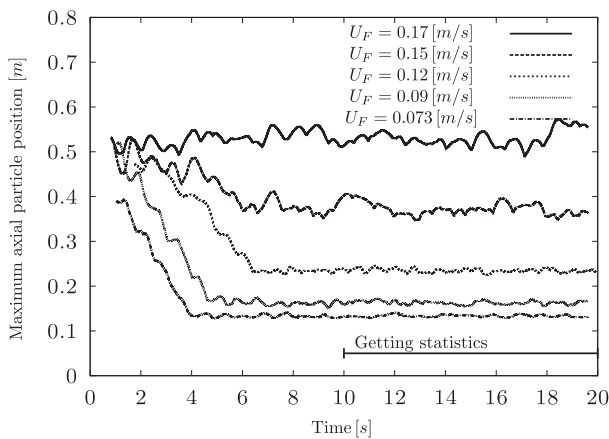
Fig. 4. Time-evolution of maximum axial particle position at different fluidization velocities: U_F = 0.17, 0.15, 0.12, 0.09, 0.073 m/s (resp. \phi_b = 0.11, 0.14, 0.22, 0.31, 0.39 ).
