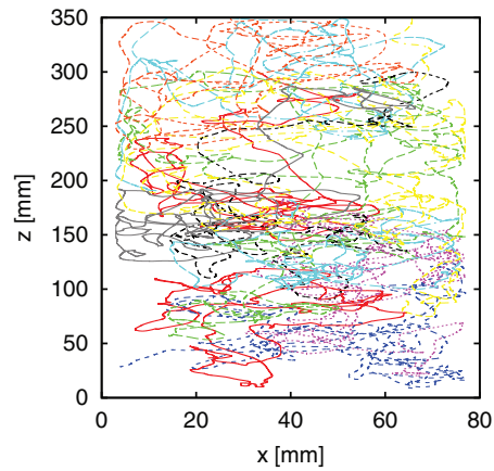
Fig. 7. Projections of particle trajectories in x - y plane (top) and x - z plane (bottom). Left: experimental data by Aguilar-Corona (2008) ( U_F = 0.15 m/s, \phi_b = 0.14 ), right: simulations.
