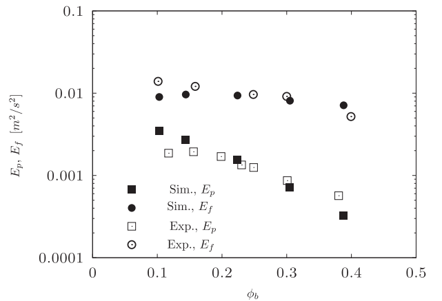
Fig. 15. Fluctuating kinetic energy of fluid phase E_f and particle phase E_p . Solid symbols: simulations, empty symbols: Aguilar-Corona (2008).
