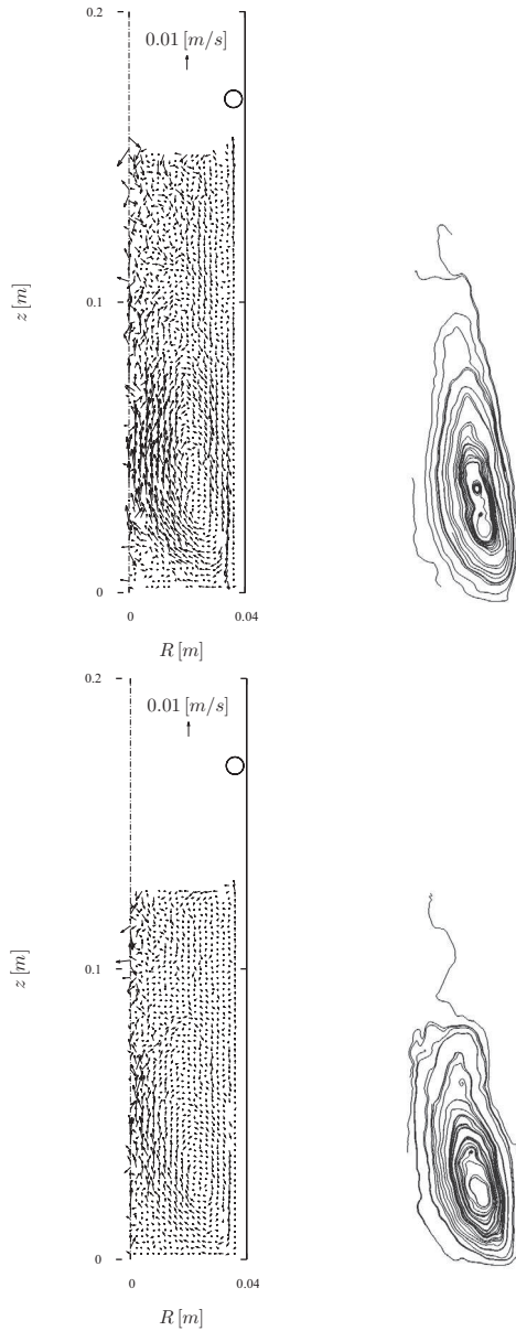
Fig. 10. Averaged particle velocity field and streamlines for the case U_f = 0.09 m/s (top) and U_f = 0.073 m/s (bottom).
