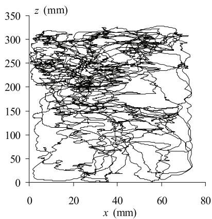
Fig. 7. Projections of particle trajectories in x - y plane (top) and x - z plane (bottom). Left: experimental data by Aguilar-Corona (2008) ( U_F = 0.15 m/s, \phi_b = 0.14 ), right: simulations.
