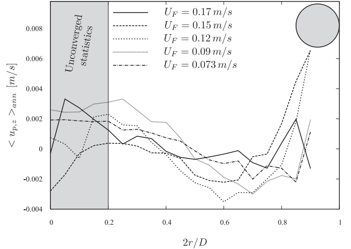
Fig. 11. Radial profile of axial velocity averaged over the bed height.
