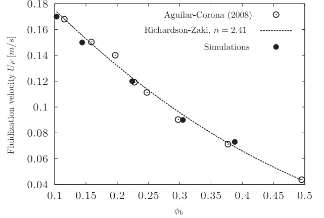
Fig. 6. Fluidization velocity with respect to the bed solid concentration. \odot : Aguilar-Corona (2008), ---: Richardson and Zaki (1954)'s correlation with n = 2.41 and \bullet : present simulations.
