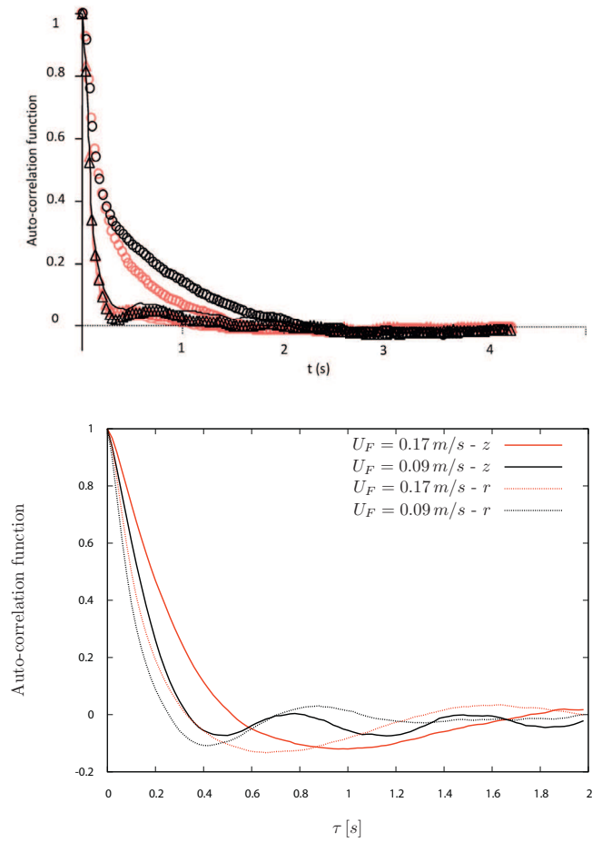
Fig. 16. Particle velocity autocorrelation functions measured in top: experiments (circles: axial component. Triangles: radial component. Black : \phi_b = 0.3 . Red= \phi_b = 0.12 ) and bottom: numerical simulation results.
