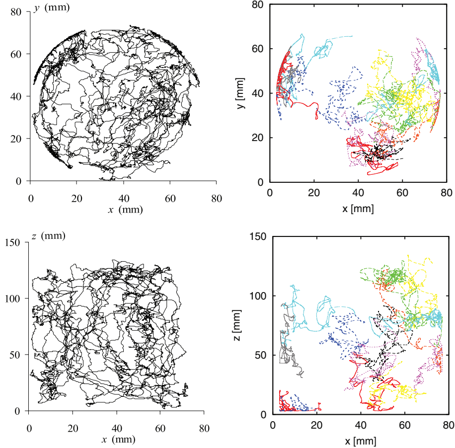
Fig. 8. Projections of particle trajectories in x - y plane (top) and x - z plane (bottom). Left: experimental data by Aguilar-Corona (2008) ( U_f = 0.073 m/s, \phi_b = 0.38 ), right: simulations.
