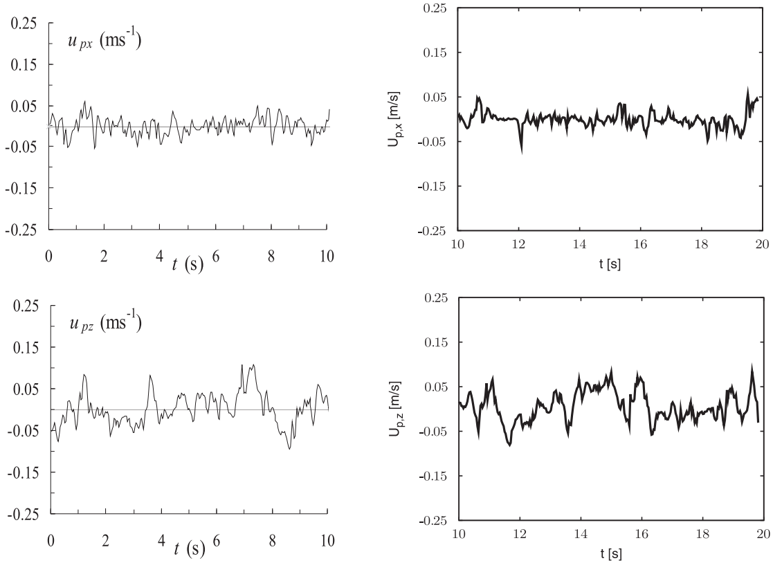
Fig. 9. Experimental data by Aguilar-Corona (2008) (left) and simulation results of a particle Lagrangian velocity signal ( \phi_b = 0.31 ; U_F = 0.09 m/s). Top: transverse and bottom: axial components.
