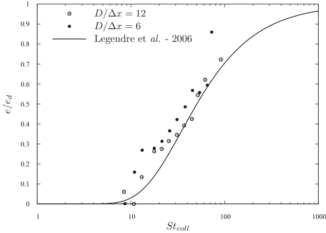
Fig. 1. Normal restitution coefficient of collisions with respect to collisional Stokes number St_{coll} = \frac{2}{9} \frac{R u_{coll} \rho_e}{\mu_f} : influence of the spatial resolution. D in this figure is the particle diameter. e is the restitution coefficient calculated from the ratio of the normal particle relative velocity before collision (at the position where lubrication force is activated) and the normal velocity after collision (where lubrication is turned off) and e_d is the reference value corresponding to collision of two glass particles.
