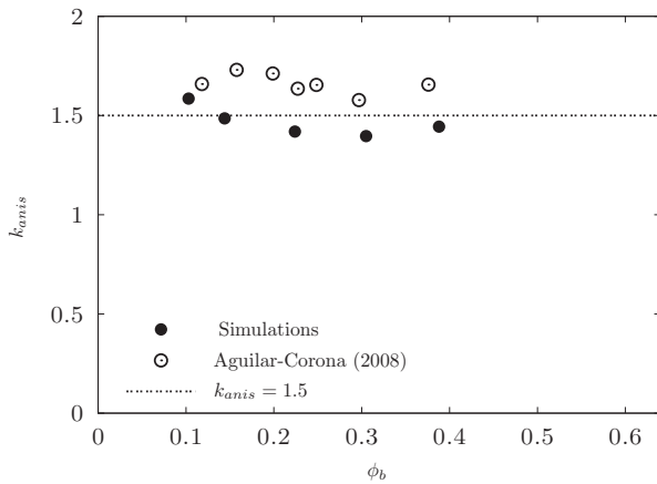
Fig. 14. Anisotropy coefficient of the particle velocity fluctuations with respect to the bed solid concentration. \odot : Aguilar-Corona (2008) and \bullet : present simulations.
