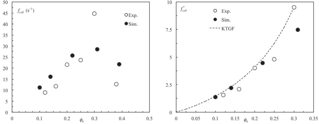
Fig. 17. Collision frequency with respect to the bed solid volume fraction (left), non-dimensional collision frequency (right) f_{coll}^* = f_{coll} \frac{d_p}{\sqrt{\frac{3}{4} (u_{p,x}^2 + u_{p,y}^2)}} compared to theoretical expression derived from KTGF f_{coll}^* = 24 \sqrt{\frac{2}{3\pi}} \phi_b g_0 with g_0 = \left(1 - \frac{\phi_b}{\phi_m}\right)^{-2.5\phi_m} and \phi_m = 0.585 .
