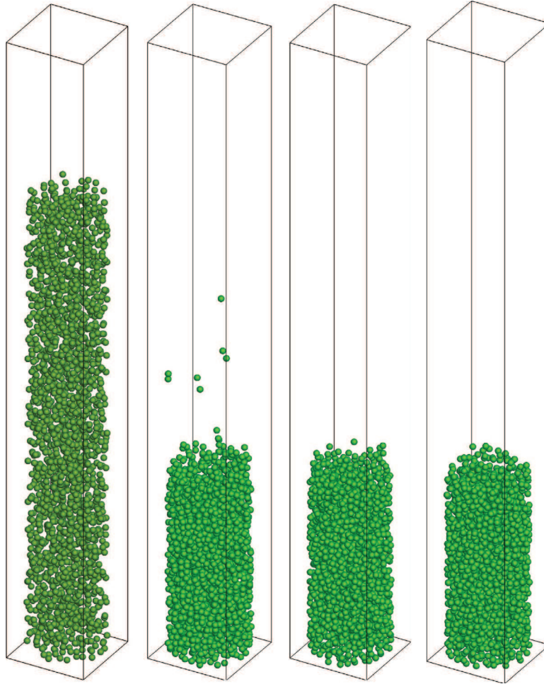
Fig. 3. 3-D views of the simulated particles inside the bed (from left to right: t = 0, 5, 10 and 20 s).
