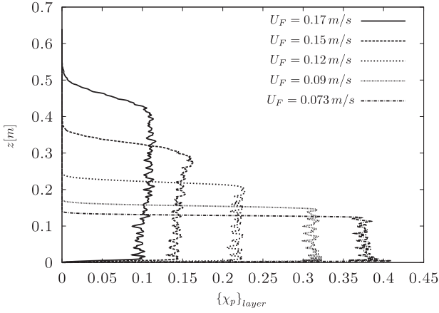
Fig. 5. Axial profile of time-section average of particle phase fraction \chi_p .
