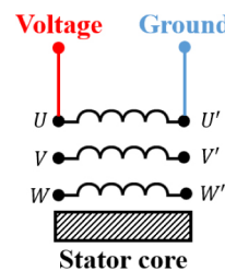
Figure 11. Schematic of coil impulse test
