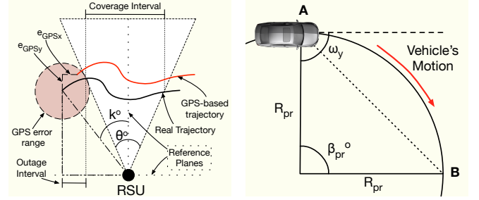
Fig. 4. a) GPS error components and the coverage and outage intervals. b) Motion of a Vehicle on the perimeter of a circle.
