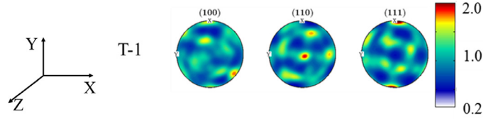
Fig. 2. The initial, relatively random, texture of the austenitic steel used in the analyses.
