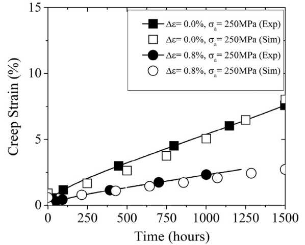
Fig. 8. The influence of prior cyclic plasticity on creep strain. The results with no cyclic pre-strain, \Delta\varepsilon = 0\% , are compared with those obtained with cyclic pre-straining. Following the pre-strain, forward creep was applied at an applied stress of 250 MPa.
