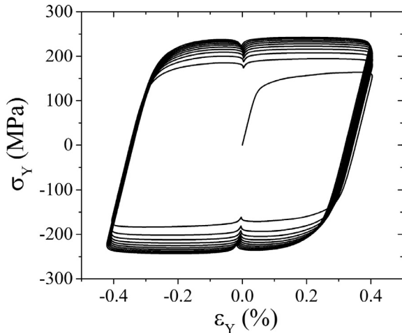
Fig. 7. Mechanical response of the CP polycrystal shown in Fig. 3 subjected to 10 cycles of \Delta\varepsilon = 0.8\% , R = -1 , uniaxial loading.
