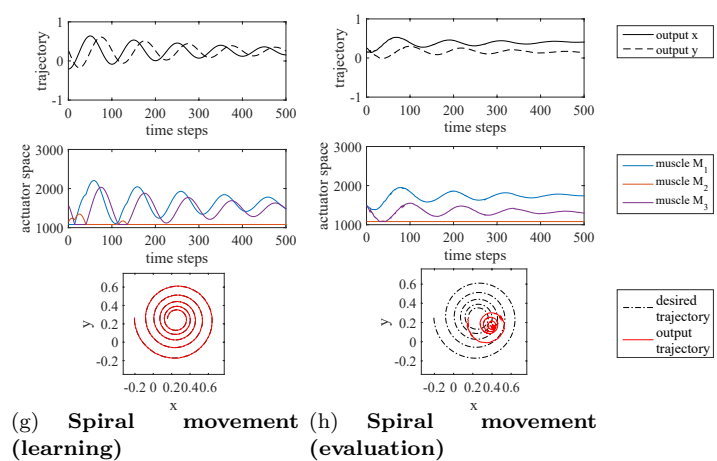
Figure 8. Results on various trajectories (linear, oval and spiral movements). Left column is the learning performance, right column is evaluation performance. The evaluation (b) of the linear movement shows that the controller is not able to handle overlapping trajectories. Introducing an additional lateral movement (oval trajectory (c,d)) solves this issue. The controller can also handle trajectories which are not limit-cycles up to a point (e,f).
