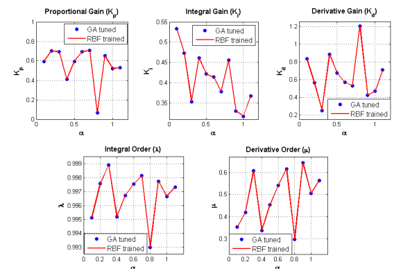
Fig. 9. Optimal FOPID controller parameters for process P4.
