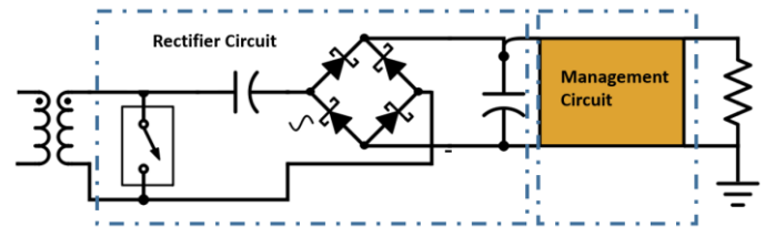
Fig. 1. A circuit diagram of the energy harvesting system.
