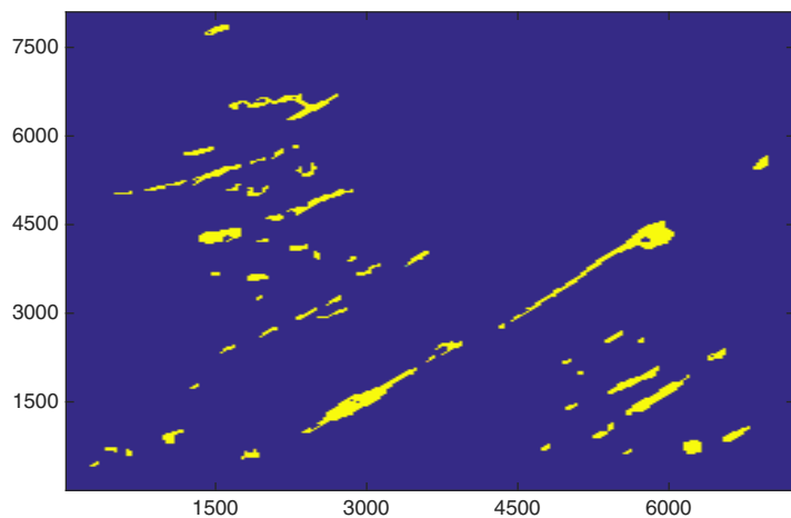
Figure 8. Landsat image of a section of the Larsen C Ice Shelf where melt lakes were present on 6 January 2016. Both axes have units of meters. Here the lakes are colored yellow and areas where lakes were not present are colored blue. Although these data were taken from the Landsat 8 mission so is from a later time than the lakes examined using the 2010–2011 melt season, it is likely that the lakes will be similar in many aspects due to the role of topography in the location of lake basins.
