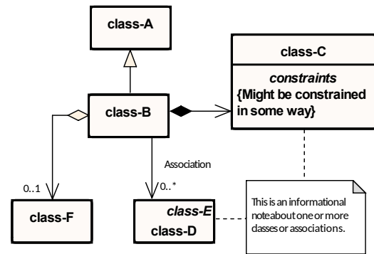
Figure A1. A worked example demonstrating the subset of UML used in this paper (see Table 1 for definitions of the class associations). Class-B is a subclass of class-A, and class-D is subclass of class-E. An instance of class-B includes one instance of class-C (that cannot exist independently) and may include zero or one instance(s) of class-F (that can exist independently). An instance of class-B is related to any number of instances of class-D (with the relationship being described by the label “Association”). An instance of class-C is constrained to exhibit some behaviour. There is a general comment concerning class-D and class-C.
