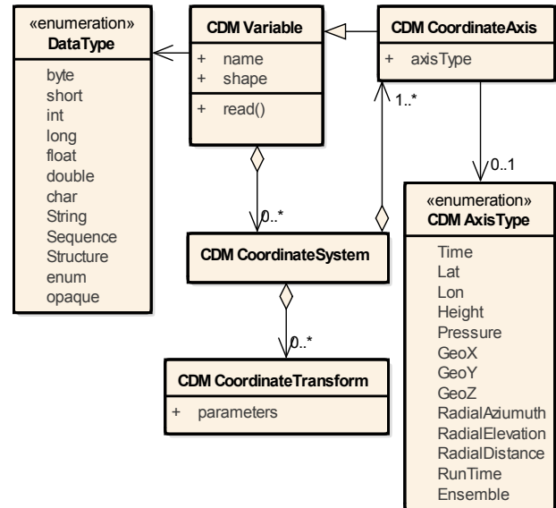
Figure 14. Key characteristics of the Unidata Common Data Model. There is a wider variety of fundamental data types than is supported by the netCDF classic data model; and the coordinate system includes the option of coordinate axes of specific types for use in the feature types, which limits the flexibility of the CDM data model.
