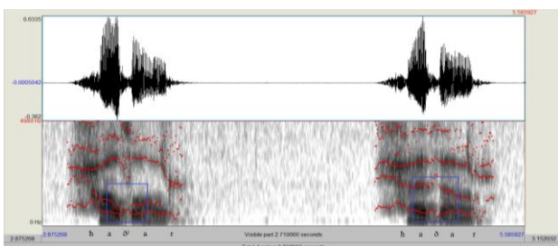
Figure 1: Praat screenshot showing differences in the vowel formants between the emphatics /ð ʕ / and non-emphatic /ð/ in a native speaker of Arabic.
