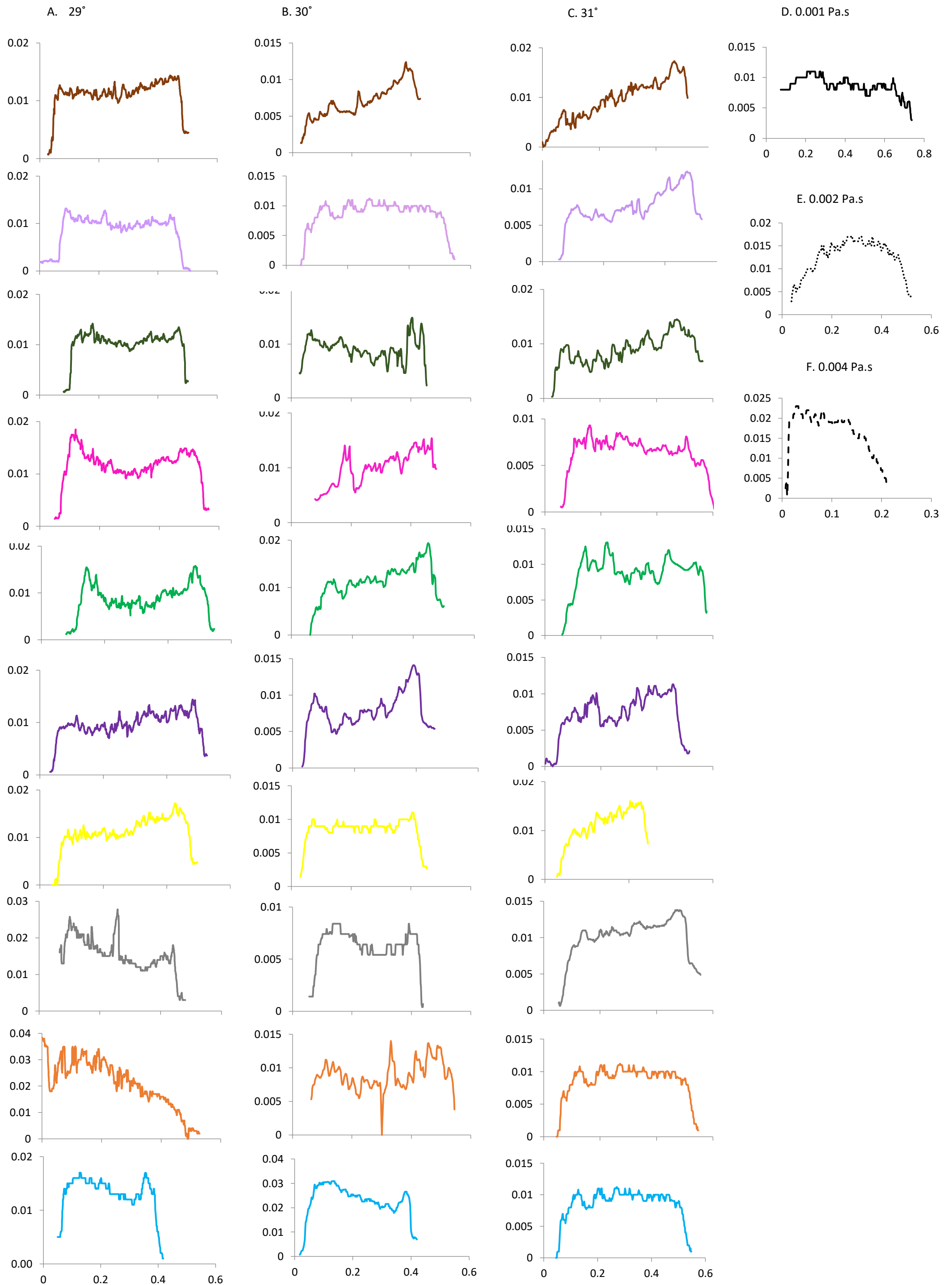
Figure 3.12. Cross-sections of the debris-flow deposits from flows at different slope angles (with viscosities of 0.0025 Pa.s): (a) 29°, (b) 30°, and (c) 31°, and at different viscosities: (d) 0.001 Pa.s, (e) 0.002 Pa.s, and (f) 0.004 Pa.s.
