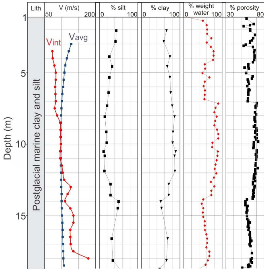
Figure 2. Shear wave velocity logs from borehole BH-NRC-MO and geotechnical data from samples collected in several boreholes around the NRC test fill. Figure adapted from Lo et al. (1976), and Hunter et al. (2010). Porosities were calculated from weight % water contents assuming a specific gravity of 2.65 for the solid and a saturation of 100%.
