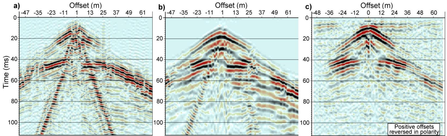
Figure 9. Comparison of seismic (a, b) and seismoelectric (c) composite shot gathers acquired using the Minivib vibroseis source with a 20 – 350 Hz sweep, subsequently highpass filtered at 200 Hz. Trace amplitudes have been normalized by their RMS values. Timing lines are 20 ms apart and offsets range from -51 to +72 m with a trace spacing of 1.5 m. Seismic results (a) and (b) differ in that 1 s AGC scaling was applied to (a) prior to vibroseis correlation in order to counteract high frequency absorption. Comparing (b) and (c) which were processed in the same way, it is again evident that the P-wave reflection from bedrock is detected sooner and exhibits broader bandwidth in the seismoelectric record.
