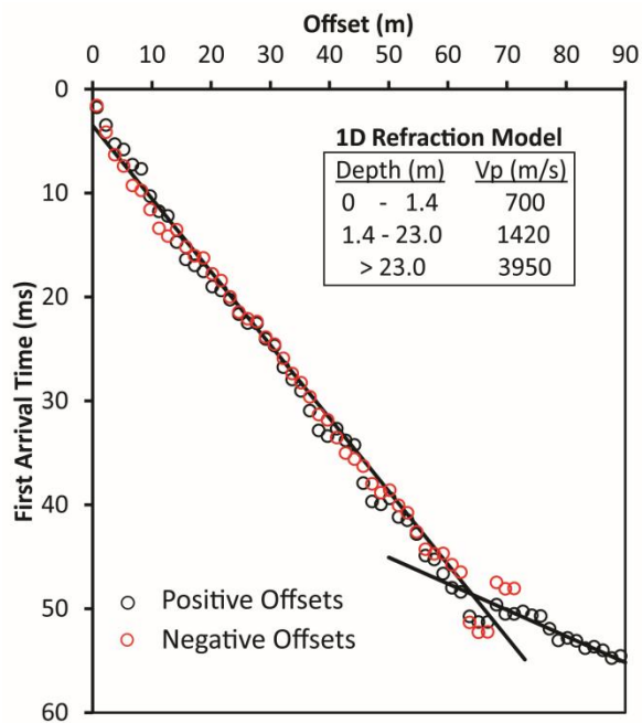
Figure 7. Analysis of first arrivals in the shotgun seismic supergather in terms of a P-wave velocity model for the site consisting of three horizontal layers. Critically refracted arrival times shown here have been increased by 1.4 ms to correct for the fact that the shotgun shell was detonated at a depth of 1 m in an upper layer.
