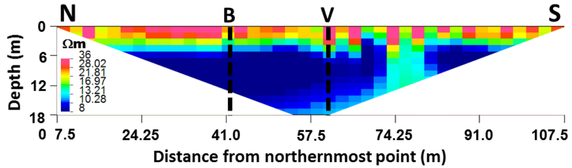
Figure 5. Resistivity section of the study site, based on a 2D ERT survey acquired with an electrode spacing of 5 m. The dashed lines show the midpoints of the buffalo gun (B) and vibroseis (V) supergatherers, as illustrated along with the ERT survey line in Fig. 1.
