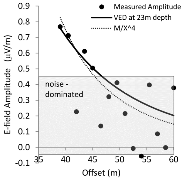
Figure 8. Amplitude of the possible interfacial seismoelectric conversion from top of bedrock (event (4) in Fig. 6(c)) plotted as a function of shot-receiver offset. The solid curve shows the rate of amplitude decay that would be expected for vertical dipole source situated at the top of bedrock 23 m below surface; at these intermediate offsets the rate of decay is nearly indistinguishable from 1/x^3 dependence, x being shot-receiver offset. For comparison, the dotted line shows the 1/x^4 amplitude dependence that would be expected at offsets much greater than the depth to the responsible interface.
