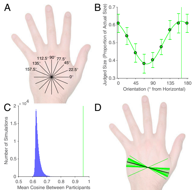
Fig. 2. ( A ) The eight stimulus orientations used in the study. ( B ) Results from Exp. 1 showing judged size as a function of stimulus orientation. The dashed green curve shows the best-fitting sinusoid. The data were fit well by this function. The vertical green line indicates the peak of the sinusoid, reflecting the orientation at which tactile distances were judged as largest (i.e., the axis in which tactile space is stretched). Error bars indicate one SE. For illustrative purposes, the same data point is shown as both 0^\circ and 180^\circ , although it was only included once in analyses. ( C ) Phase alignment of best-fitting curves. The green vertical line indicates the mean cosine of the angular deviation between each pair of the 25 participants. The blue histogram shows the same mean calculated for each of 1 million simulations of random data. The green vertical line was larger than any of the simulations, indicating that the phase alignment in the data was greater than would be expected by chance. ( D ) The axis of stretch. Each green line indicates the orientation of maximal stretch for a single participant. The black line indicates the average axis across participants.
