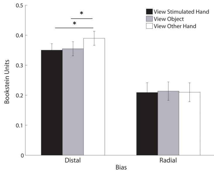
Figure 7. Distal and radial bias in the three experimental conditions. Error bars indicate the standard errors of the mean ( \pm SEM). *denotes p < 0.05 .
