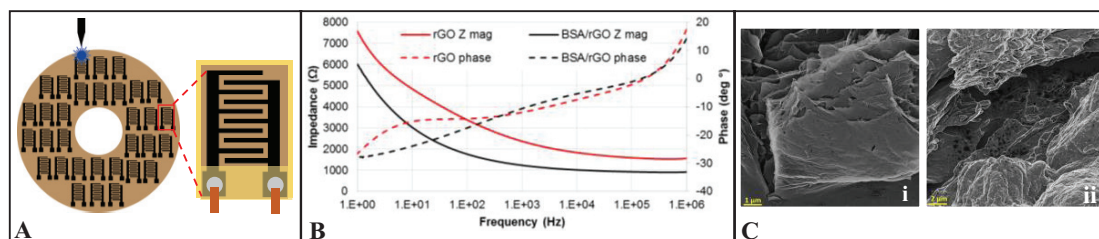
Figure 1: A) Lightscribe rGO production process and IDE diagram; B) Bode plot (impedance magnitude and phase) for the rGO biosensing platform before and after BSA immobilization; C) HIM image of (i) rGO and (ii) rGO after electroless nickel metallization.
