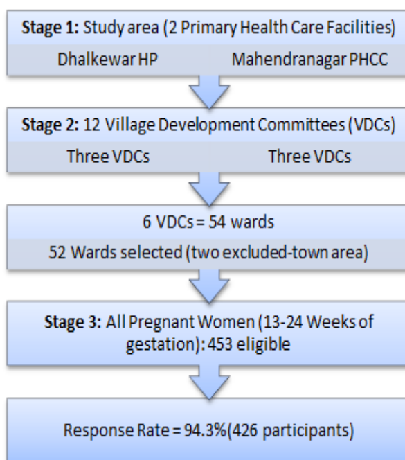
Figure 1. Sampling Strategy
