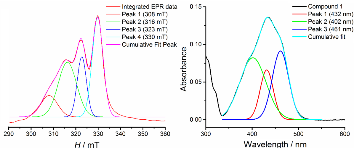
Figure 11 left: Integrated and deconvoluted EPR data for a 1 \times 10^{-2} M solution of 1 in DMSO at 293 K (peak 1 is from a DMSO-solvated free Cu(II) ion); right: Deconvoluted UV-vis data for a 1 \times 10^{-5} M solution of 1 in DMSO.
