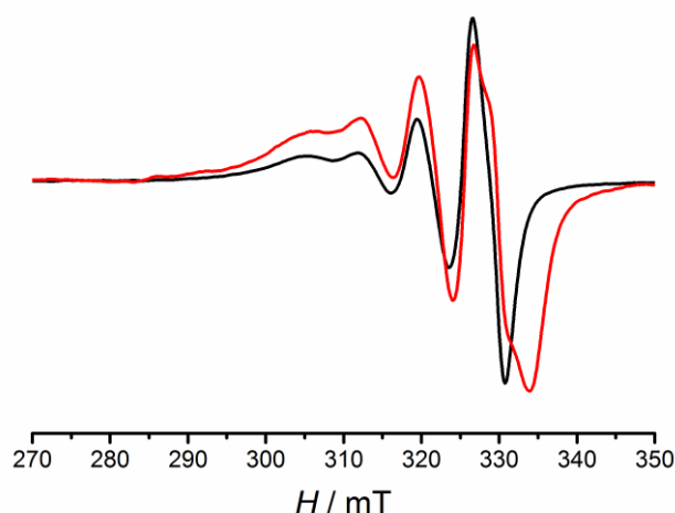
Figure 12 Comparison of EPR spectra of a 1 \times 10^{-2} M solution of 1 (black line) and 2 (red line) in DMSO at 293 K.
