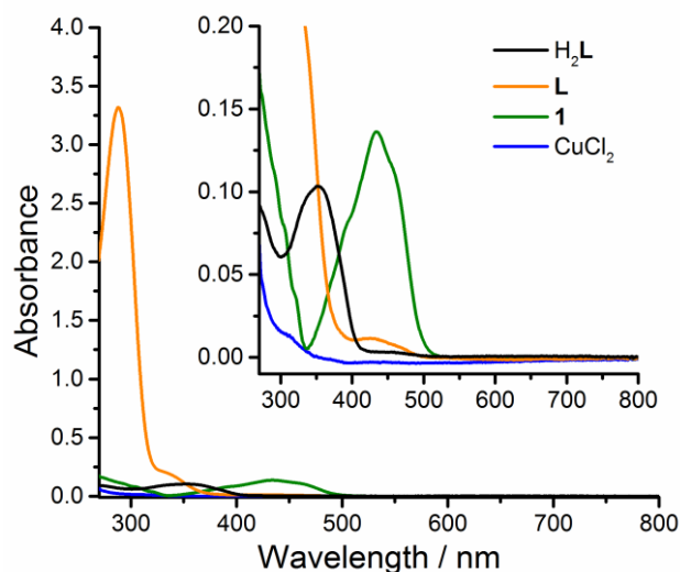
Figure 10 UV-vis spectroscopy of 1 \times 10^{-5} M solutions of a) H_2L in DMSO (black); b) L^{2-} in 5% NEt_3 in DMSO (orange); c) compound 1 in 5% NEt_3 in DMSO (green) and d) CuCl_2 \cdot 2H_2O in 5% NEt_3 in DMSO (blue).
