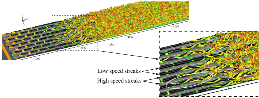
Fig. 8: Iso-surfaces of Q (=200) coloured with axial velocity for test case k8 . Iso-surfaces of streamwise velocity fluctuation u' are also overlaid. Positive perturbation ( u' = 0.2U_\infty ) represented by light grey and negative perturbation ( u' = -0.2U_\infty ) indicated by black. Inset plot shows the magnified view of the transition zone and evolution of hairpin vortices.
