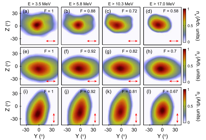
Figure 3. Measured electron density distribution. (a–d) Electron density as measured using IP for l = 800 nm, for electrons with energy greater than: (a) 3.5 MeV; (b) 5.8 MeV; (c) 10.3 MeV; and (d) 17.0 MeV; all for linear polarization in the Y -axis. (e–h) Same for l = 40 nm and linear polarization in the Y -axis. (i–l) Same for l = 40 nm and linear polarization in the Z -axis. The colour maps are scaled by the stated value F to clearly show the features of interest at each energy slice. The red arrows show the laser polarization.
