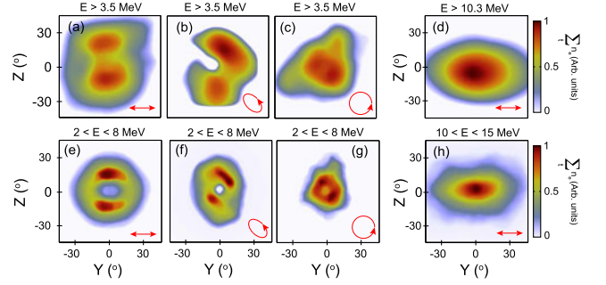
Figure 5. (a) Electron density for a l = 10 nm target as measured using IP for electrons with energy greater than 3.5 MeV for linear polarization. (b) Same for elliptical polarization. (c) Same for circular polarization. (d) Same as (a) but for a l = 40 nm target with energy greater than 10.3 MeV. (e)–(g) 3D PIC simulation results for the electron density distribution from l = 10 nm and energies 2 < E < 8 MeV for linear, elliptical and circular polarization, respectively. (h) Same but from l = 40 nm and energies 10 < E < 15 MeV and linearly polarized light. The red arrows show the laser polarization.
