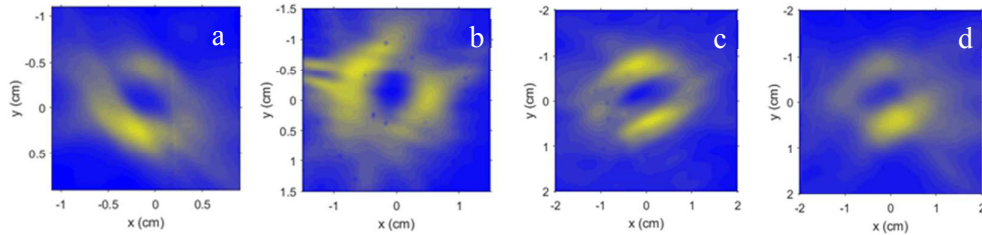
Figure 4. Beam profiles recorded for the beams generated using (a) circular ( l = 0 ), (b) 1-arm ( l = 1 ), (c) 2-arm ( l=2 ) and (d) 3-arm spiral gratings.
