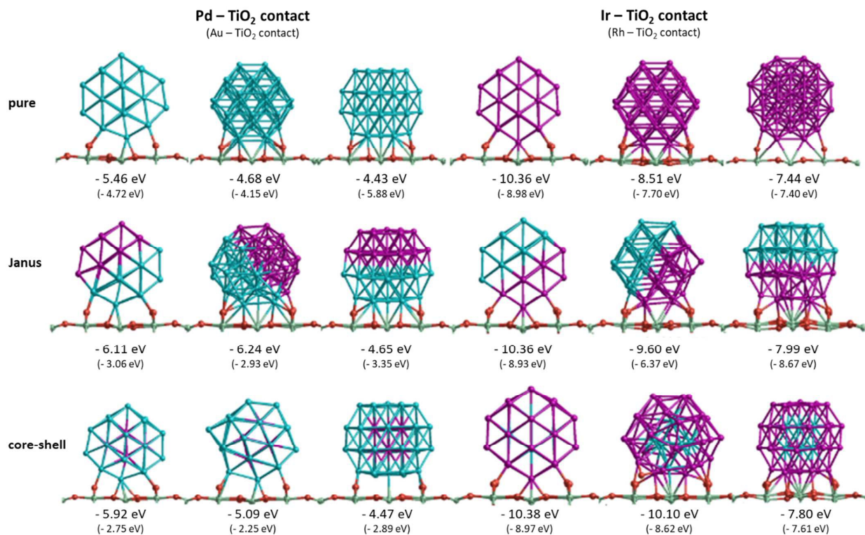
Figure 5. Structures and corresponding surface binding energies ( E_{s\text{-bind}} ) for 38-TO pure Pd and Ir clusters and Pd-Ir nanoalloys supported on \text{TiO}_2(110) in three orientations. The surface binding energies of Au-Rh clusters, corresponding to the same structures (with Au replacing Pd and Rh replacing Ir), are given in parentheses. Pd, Ir, O and Ti atoms are represented in blue, purple, red and green, respectively. For simplicity, only the top layer of the \text{TiO}_2 slab is shown.
