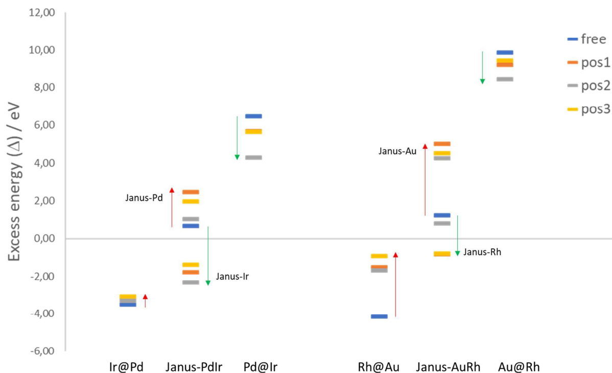
Figure 6. Excess energies of free and \text{TiO}_2 -supported Pd-Ir and Au-Rh 38-TO clusters with core-shell (A@B) and Janus configurations. The coloured bars represent the free NP and the three different binding positions on the support.
