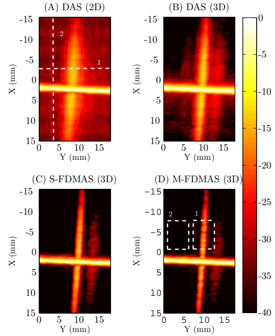
Fig. 3: The photoacoustic images for carbon fibre rods (A) based on DAS(2D) , (B) DAS(3D) (C) S-FDMAS(3D) and (D) M-FDMAS(3D) (-40 dB Dynamic range).
