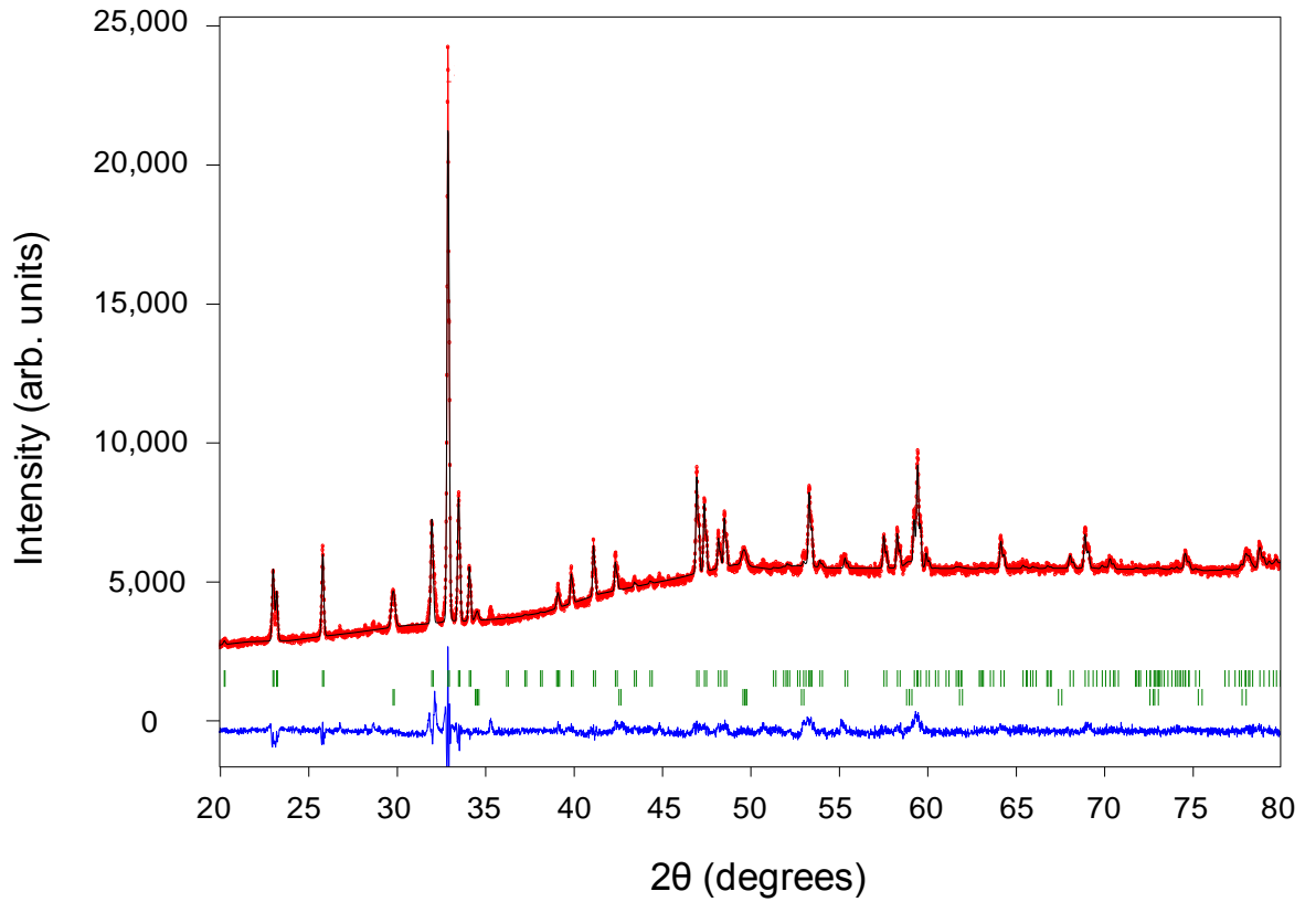
Figure 5. X-ray diffractogram of \text{GdFeO}_3 with Rietveld refinement using \text{GdFeO}_3 and \text{ZrO}_{1.97} starting structures. Red line indicates observed data, black line indicates calculated data, blue line shows difference between observed and calculated data. Green lines indicate the positions for \text{GdFeO}_3 (upper) and \text{ZrO}_{1.97} (lower).
