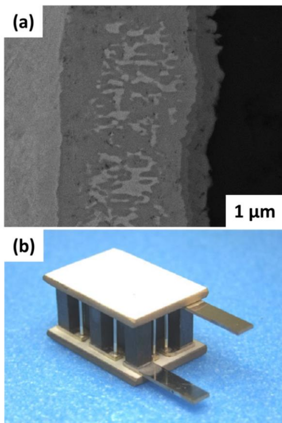
Figure 10. (a) Secondary electron image of a Ni/Mg 2 Si interface after sintering for 15 min at 1023 K 123 , showing pure Ni as a bright phase on the left, Mg 0.52 Ni 0.48 Si 4 in darker grey and Mg 2 Si in black. (b) Unileg device, consisting of ten thermoelectric legs of Sb-doped Mg 2 Si legs 133 .
