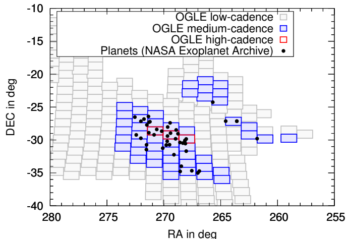
Fig. 7. Number and location of planets confirmed by 2017 (NASA Exoplanet Archive) is shown along with the survey cadence.
