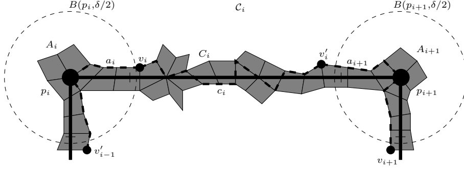
FIGURE 11.4. Construction of the curve \mathcal{C}' .
