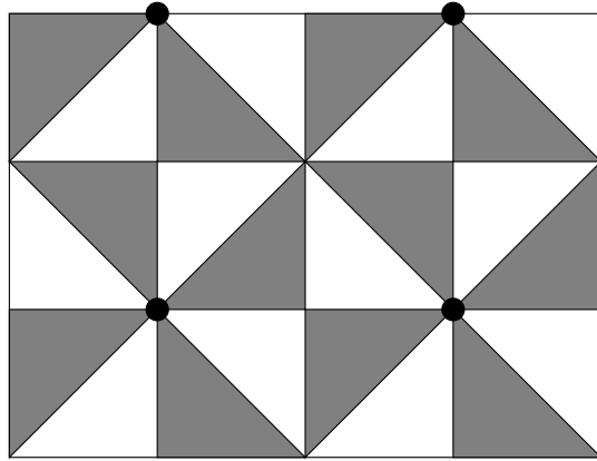
FIGURE 3.1. Invariant tiling for type (244).
