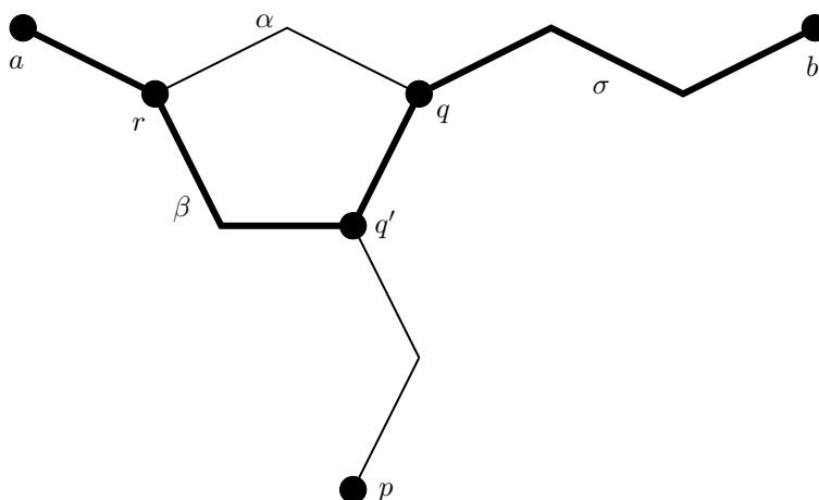
FIGURE 11.3. Constructing a path through a, b, p .
