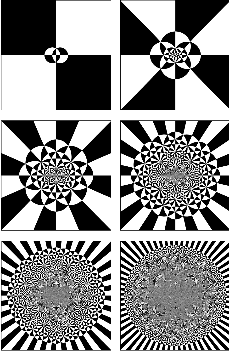
FIGURE 12.7. Tiles of levels 1–6 for the barycentric subdivision map f_2 .
