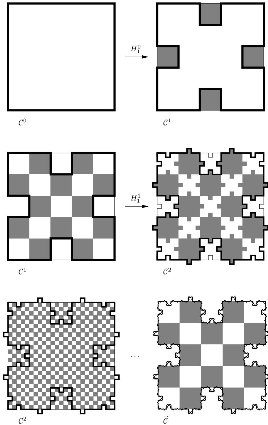
FIGURE 15.4. Iterative construction of an invariant curve.
