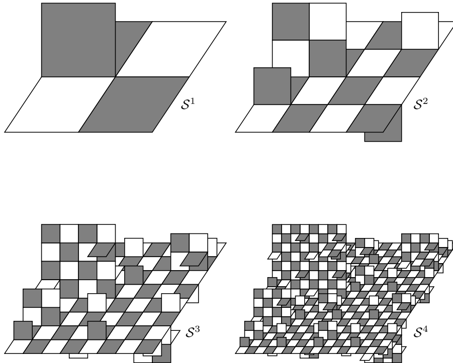
FIGURE 1.3. Polyhedral surfaces obtained from the replacement rule.
