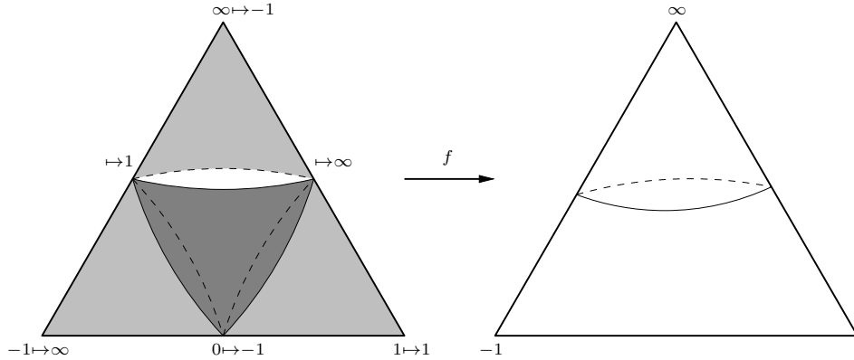
FIGURE 3.7. A Lattès map with orbifold signature (3, 3, 3) .
