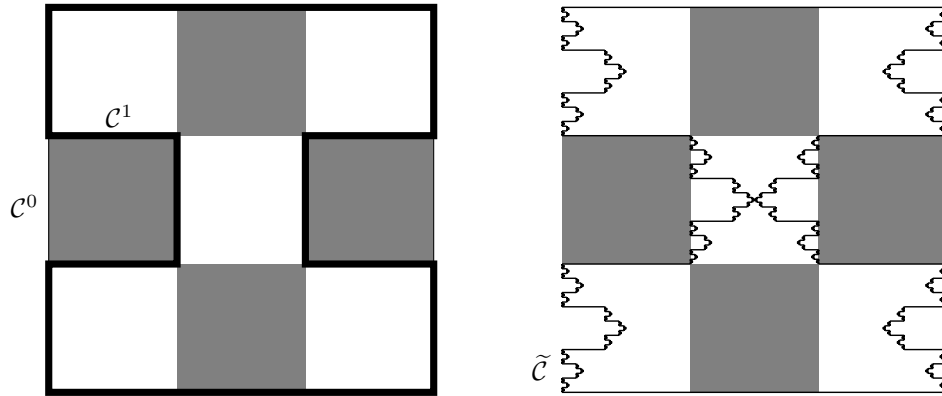
FIGURE 15.6. Since \hat{g} is not combinatorially expanding, \tilde{C} is not a Jordan curve.
