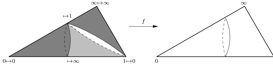
FIGURE 3.8. A Lattès map with orbifold signature (2, 3, 6) .
