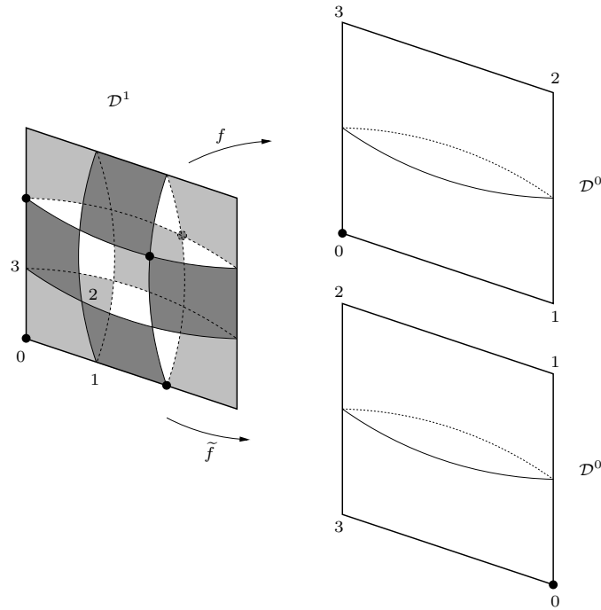
FIGURE 12.3. Two subdivision rules.
