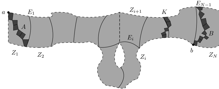
FIGURE 20.1. The setup in Lemma 20.12.
