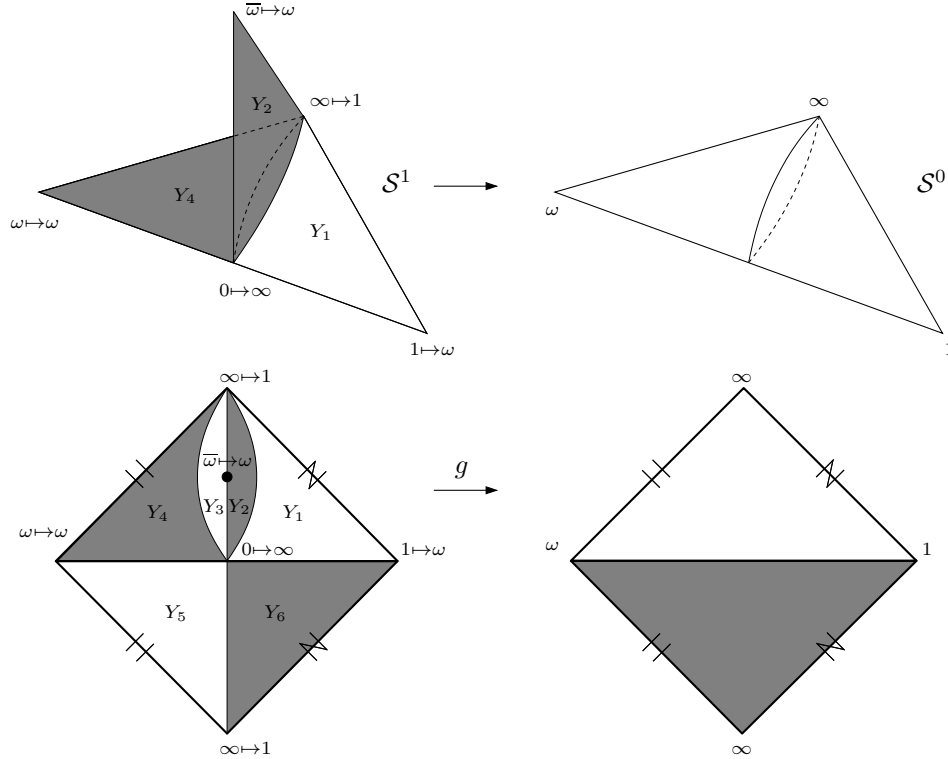
FIGURE 2.1. The map g .
