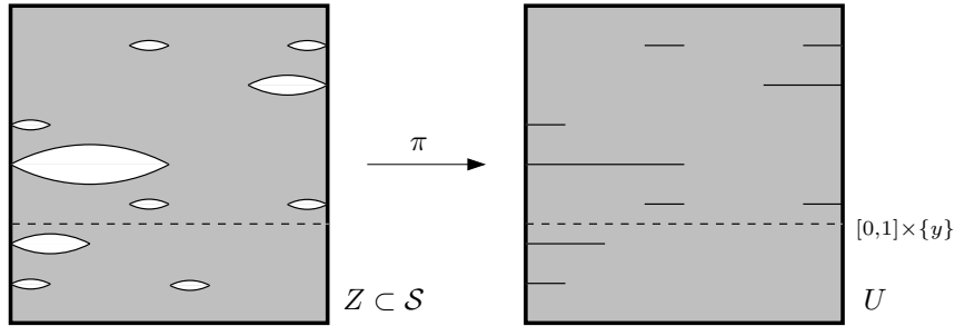
FIGURE 4.2. The set Z .
