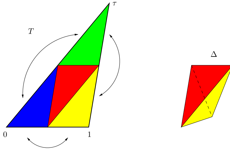
FIGURE 3.4. Folding a tetrahedron from a triangle.
