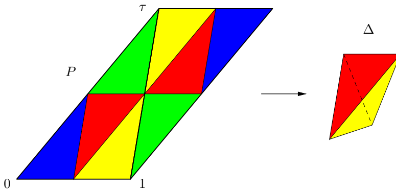
FIGURE 3.5. Construction of \Theta = \varphi .
