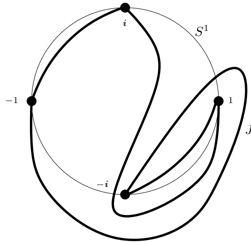
FIGURE 11.2. J is not isotopic to S^1 rel. \{1, i, -1, -i\} .
