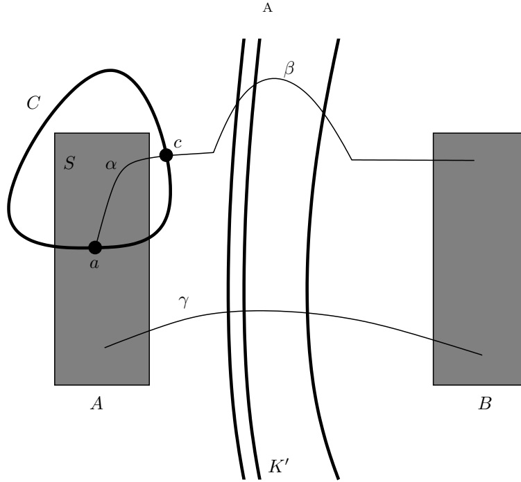
FIGURE A.1. Proof of Lemma A.4.
