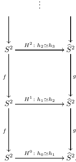
FIGURE 11.1. Tower of isotopies.
