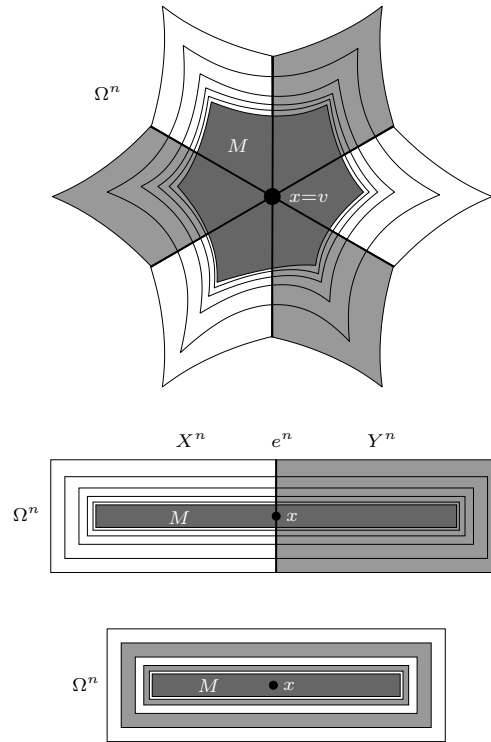
FIGURE 14.1. Equivalence classes of vertex-, edge-, and tile-type.
