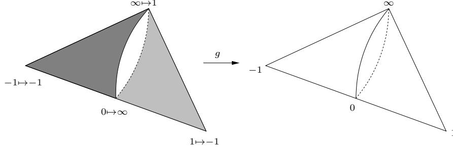
FIGURE 3.6. A Lattès map with orbifold signature (2, 4, 4) .
