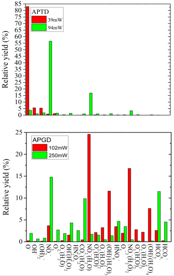
Figure 8 a) and 8b). Mass spectra for negative ions present in helium a gas flow rate 2.0 slm a) sinusoidal APTD for low and high power case and b) pulsed APGD for low and high power case.
