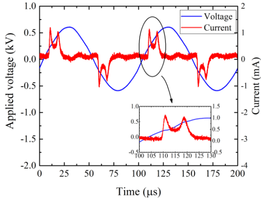
(a) sine-wave at V_{pp}=1.2kV , f=10kHz
