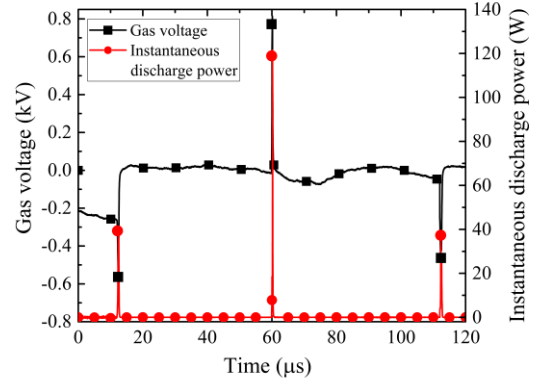
(b) unipolar square-wave at V_{pp}=1.15kV , f=10kHz
