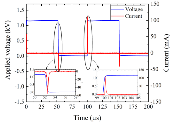
(b) unipolar square-wave at V_{pp}=1.15kV .
