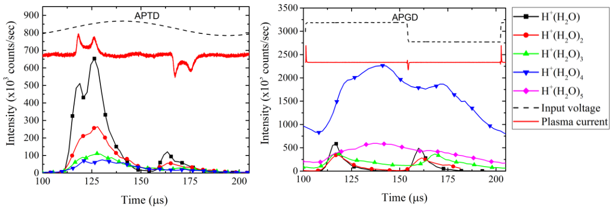
Figure 7a) and 7b). Time-resolved mass spectrometry data of water cluster ions a) APTD, and b) APGD
