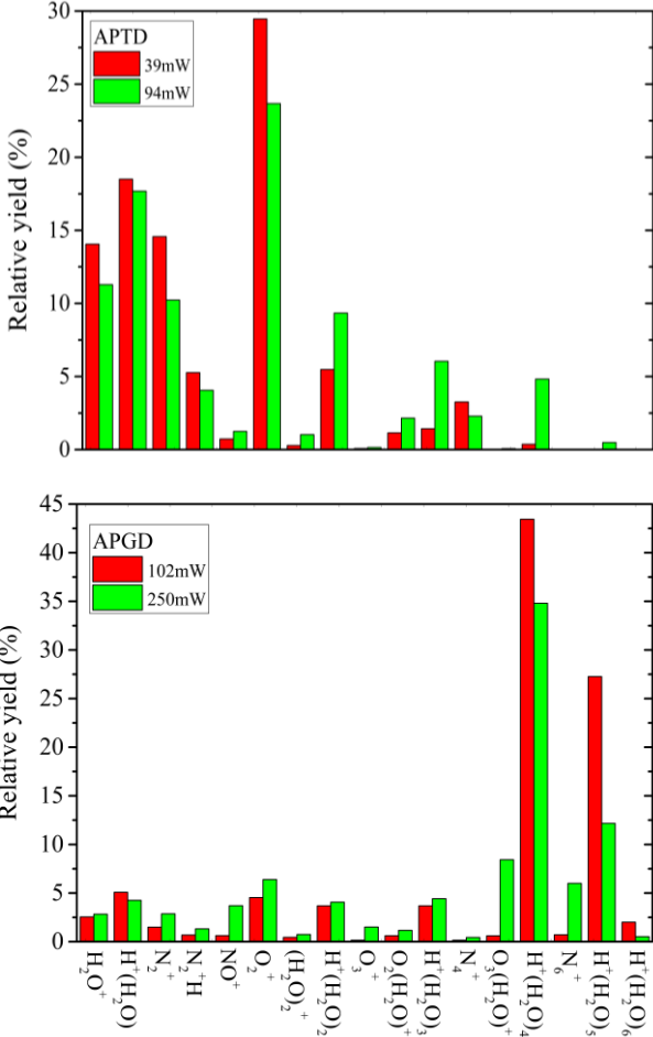
Figure 5 a) and 5b). Mass spectra for ions present in helium a gas flow rate 2.0 slm a) sinusoidal APTD for low and high power case and b) pulsed APGD for low and high power case.
