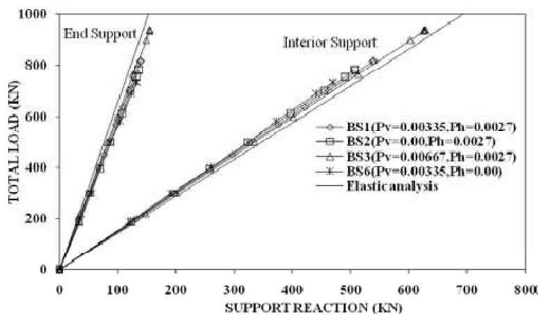
Fig. 10. Total Applied Load versus Support Reactions for Beams Having ( a/d = 1.0 )
