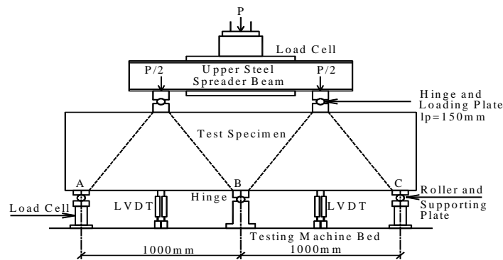
Fig. 3. Typical test setup and instrumentation for all tested beams
