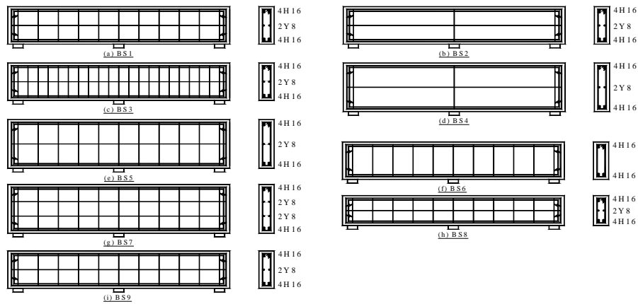
Fig. 2. Details of Tested RC Deep Beams
