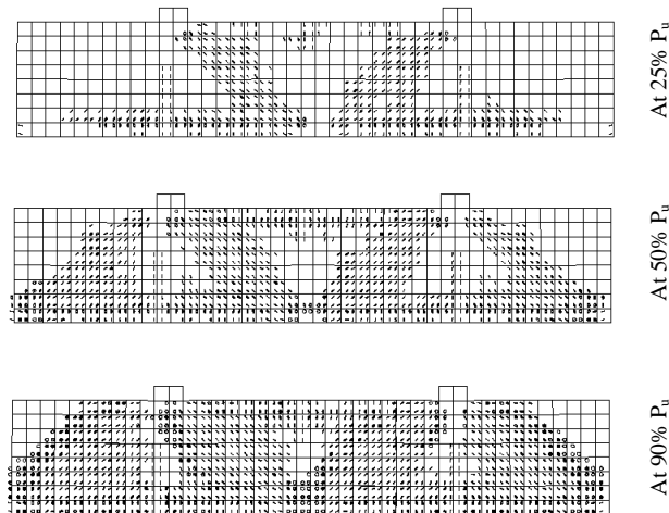
Fig. 12. Simulated Crack Propagation for Tested Beam BS8
