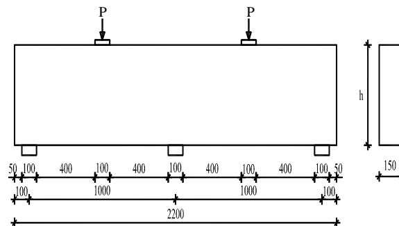
Fig. 1. Geometrical Dimensions of the Tested Deep Beams (mm)
