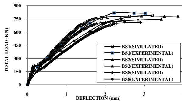
Fig. 13. Simulated and experimental load-deflection curves for BS1, BS2, and BS8
