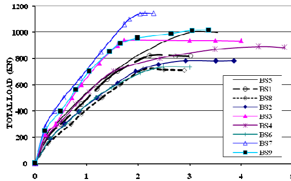
Fig. 5. Total Applied Load and Mid-Span Deflection Relationship for the Tested Beams
