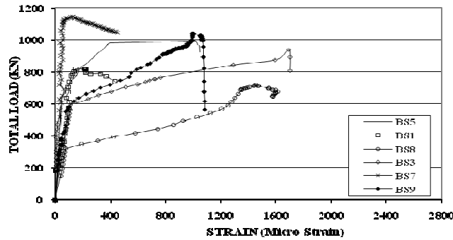
Fig. 8. Total Applied Load and Vertical Shear Reinforcement Strain Relationship
