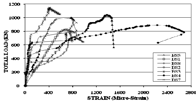
Fig. 9. Total Applied Load and Horizontal Shear Reinforcement Strain Relationship
