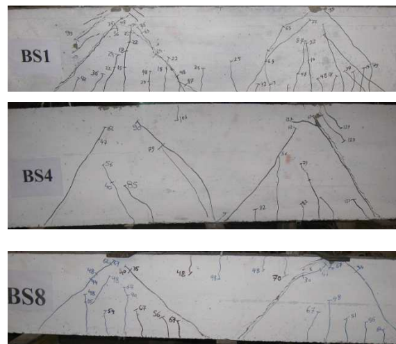
Fig. 4. Crack Patterns and Failure Zones of Tested Beams BS1, BS4, and BS8
