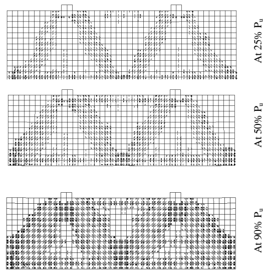
Fig. 11. Simulated Crack Propagation for Tested Beam BS5
