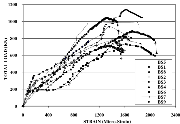
Fig. 6. Total Applied Load and Bottom Steel Strain Relationship for the Tested Beams
