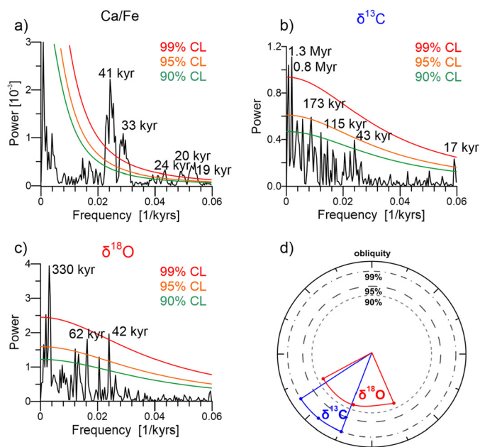
Fig. 3. Spectral and phase analysis of proxy records. Redfit power spectra of the a) Ca/Fe, b) \delta^{13}\text{C}_{\text{benthic}} , and c) \delta^{18}\text{O}_{\text{benthic}} . Main periods are highlighted. d) Phase wheel illustrating the phase relations between benthic foraminiferal stable isotopes and Ca/Fe at the obliquity band (41 kyr). In the phase wheel representation, vectors in the 12 o'clock position are in phase with maximum Ca/Fe, and phase lags increase in the clockwise direction (for example, 3 o'clock represents a 90° lag relative to Ca/Fe, 6 o'clock represents an antiphase response, and 9 o'clock represents a 90° lead). Vector length (from circle centre to middle of arc) represents coherence, and the associated arc denotes the phase within 2\sigma phase error. Circles mark 99% (dashed-dotted), 95% (dashed) and 90% (dotted) coherence.
