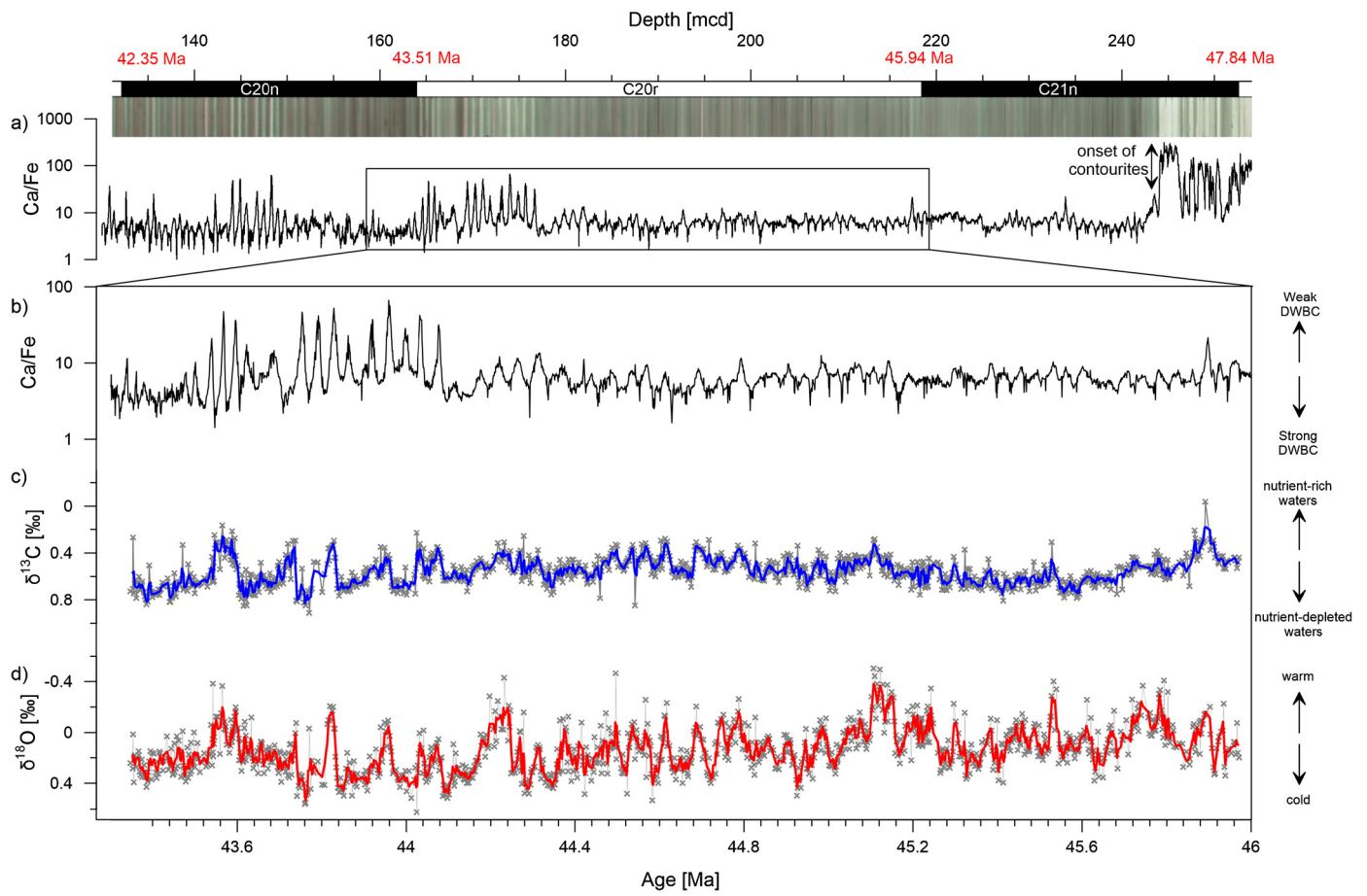
Fig. 2. Obliquity-paced paleoceanographic proxy records from IODP Site U1410. (a) XRF-derived Ca/Fe indicate the onset of drift sedimentation at 244 mcd. (b–d) Ca/Fe, \delta^{13}\text{C}_{\text{benthic}} and \delta^{18}\text{O}_{\text{benthic}} records of chron C20r in the time domain. We consider C20r boundary ages of 43.51 and 45.94 Ma and apply linear interpolation in between these tie-points, so to convert depth into time. Blue and Red lines on the isotopic curves represent the 6-kyr running averages. (For interpretation of the references to colour in this figure legend, the reader is referred to the web version of this article.)
