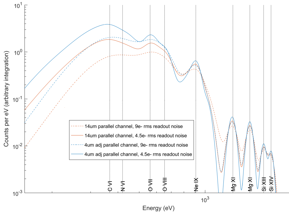
Figure 7. The spectral performance of the device is considered for this single radiation dose level across the best-case and worst-case pixel designs (14 \mu\text{m} and 4 \mu\text{m} adj) and output amplifiers (readout noise of 9 electrons rms and 4.5 electrons rms). The improvements to the both spectral line width (and therefore how resolvable the lines are) and the total count rates can be compared.
