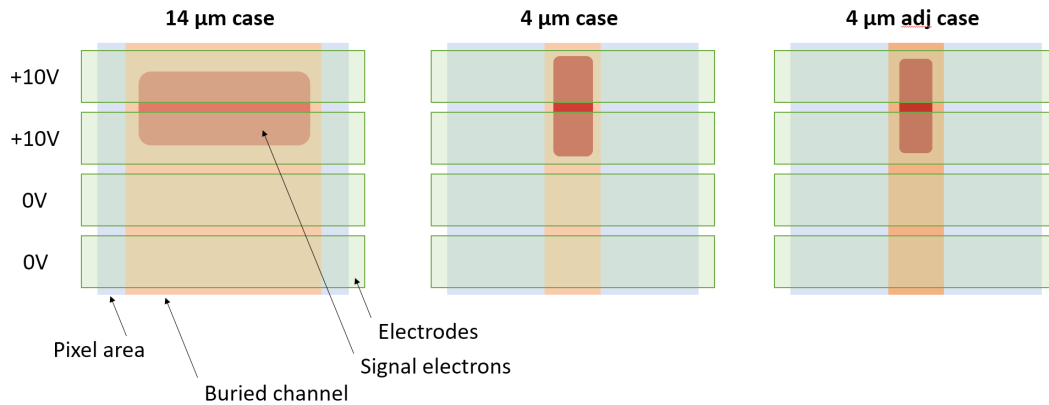
Figure 3. A cartoon of the three different cases considered, showing the 14 \mu\text{m} case and the two versions of the 4 \mu\text{m} channels. The difference between the 4 \mu\text{m} case and the 4 \mu\text{m} adj case is only the dopant concentration in the channel (changed to provide the same depletion depth as the 14 \mu\text{m} case in the adj geometry).
