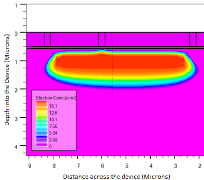
Figure 1. A side-on view of the electron density from a cut-plane through the pixel (adapted from [18]).
