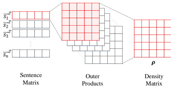
Figure 1: Single Sentence Representation
