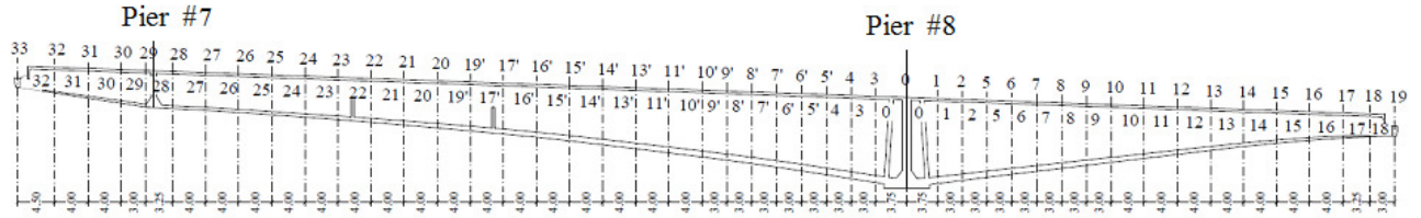
Figure 10. Discretization of the box girder under exam
