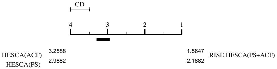
Fig. 10. A pairwise critical difference diagram of RISE and the full series spectral approaches over 100 resamples of the 85 UCR/UEA datasets
