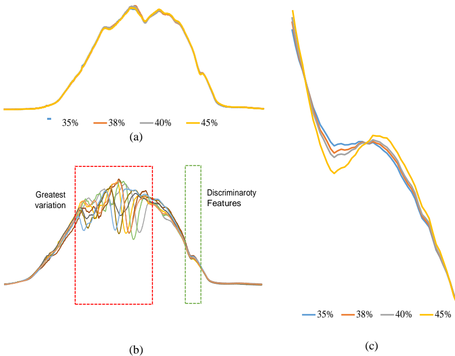
Fig. 4. Examples from the EthanolLevel problem. Part (a) shows there is little difference between the average profiles of each class, and (b) demonstrates the greatest variation between example series of different classes seems to be in the middle of the series. Expert knowledge suggests that discriminatory features will be in a band towards the end of the series however. Part (c) expands the interval from (a) and shows there is a clear difference between the average class profiles when focusing only on this specific part of the series.
