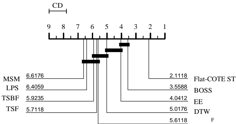
Fig. 2. The critical difference diagram of the top 9 classifiers taken from (Bagnall et al. 2016): Flat-COTE, ST (Shapelet Transform Ensemble), BOSS (Bag-of-SFA-Symbols), EE (Elastic Ensemble), DTW (DTW Features), TSF (Time Series Forest), TSBF (Time Series Bag-of-features), LPS (Learned PaNern Similarity), and MSM (Move-Split-Merge).
