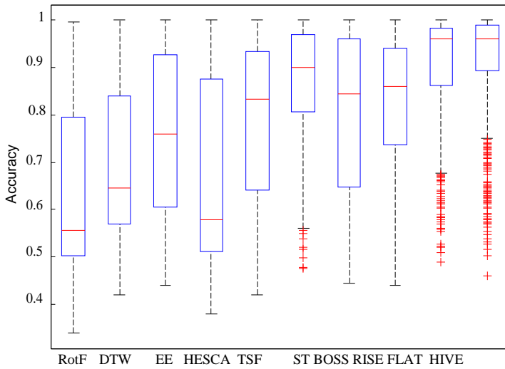
Fig. 19. Box plot of accuracies of ten classifiers over 1000 simulations.
