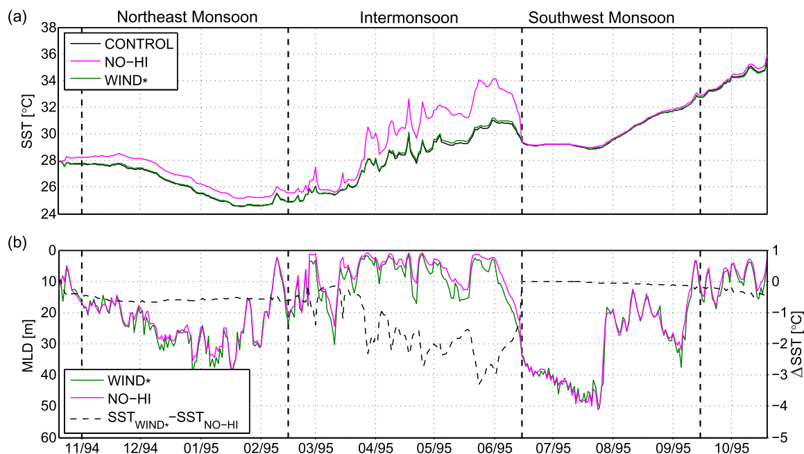
Figure 6. (a) Daily-mean SST from the CONTROL (black), NO-HI (magenta), and WIND* (green) experiments. (b) Daily-mean ML depth in the NO-HI and WIND* experiments and daily-mean SST difference (dashed) between the two experiments (WIND* – NO-HI).
