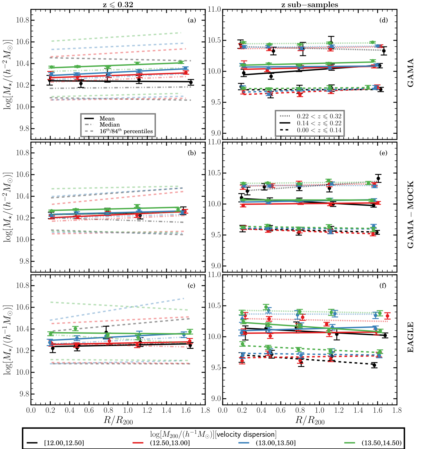
Figure 4. Stellar mass distributions of satellite galaxies in the galaxy group catalogues taken from GAMA (top row), GAMA-Mock (middle row), and EAGLE (bottom row). In all panels, different colours represent different halo-mass range. The left-hand column shows the radial runs of the central-tendency of \log(M_*) of the galaxies in galaxy groups of different halo-mass ranges for z \in (0.00, 0.32] with \log(M_*) \geq 10.0 . Means of the \log(M_*) are shown with solid lines and medians are shown with faint dash-dotted lines whereas the faint dashed lines above(below) the solid lines are the 84th(16th) percentile of the \log(M_*) in a given data range. The column in the right-hand side shows expectations of \log(M_*) in different redshift sub-samples as a function of halo mass. Here, the dashed, solid, and dotted lines represent means of the \log(M_*) in z \in (0.00, 0.14] with \log(M_*) \geq 9.1 , z \in (0.14, 0.22] with \log(M_*) \geq 9.7 and z \in (0.22, 0.32] with \log(M_*) \geq 10.0 , respectively.
