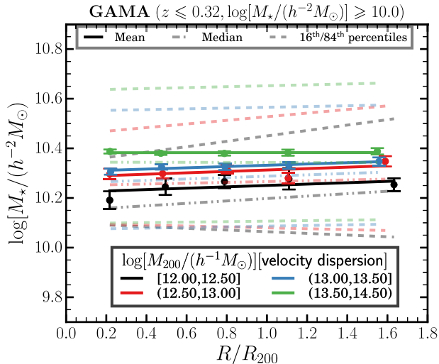
Figure 7. Stellar mass distribution of the satellite galaxies in GAMA galaxy groups with luminosity weighted centre. All labellings are identical to Fig. 4(a).
