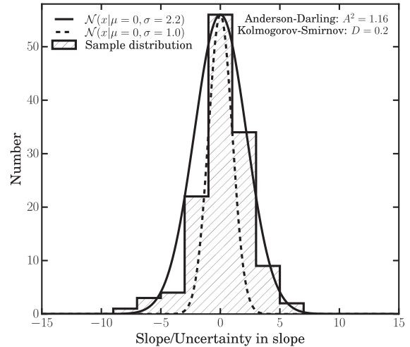
Figure 9. Distribution of the slopes of the mass segregation trend lines normalized by the estimated error. The solid and dashed lines are normal distributions with different values for dispersions overlaid for a reference.
