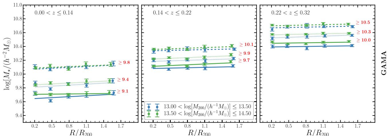
Figure A1. Effect of stellar mass completeness limits on GAMA data at three different redshift ranges, namely 0 < z \leq 0.14 (left-hand panel), 0.14 < z \leq 0.22 (mid-panel) and 0.22 < z \leq 0.32 (right-hand panel) in the two most massive halo-mass bins. The red texts shown alongside the mass segregation trends are the corresponding stellar mass limits applied to each sub-sample.
