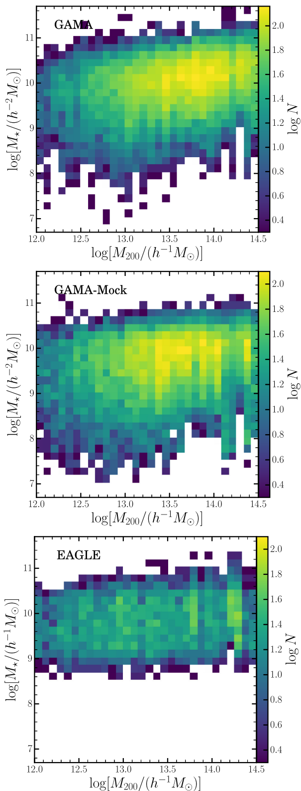
Figure 2. Stellar mass ( M_* ) of the satellites versus the host halo mass ( M_{200} ) as labelled in each panel from top to bottom is GAMA, GAMA-Mock, and EAGLE data. The colour of each pixel represents log number count of galaxies as labelled in the colour bar alongside. Note, this shows the entire sample for all the three data sets and is not just limited to the stellar mass complete sample.
