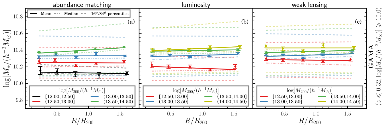
Figure 6. Stellar mass distribution of the satellite galaxies in GAMA galaxy groups in different halo-mass ranges for three halo-mass definitions (a) abundance matching, (b) luminosity based, and (c) weak lensing. All labellings are identical to Fig. 4(a), but note largest halo-mass bin further split into two bins (13.50,14.00] and (14.00,14.50).
