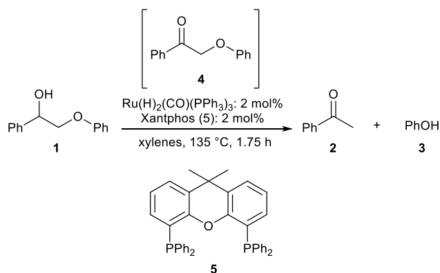
Scheme 1: C-O bond cleavage in 2-phenoxy-1-phenylethanol ( 1 ) by (\text{Ru})(\text{H})_2(\text{CO})(\text{PPh}_3)_3 -Xantphos catalyst studied by Berman, Ellman and co-workers. 32
