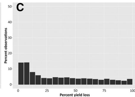
Fig. 6. An illustration of the impact of including expert opinion about the frequency distribution of resistance deployment, compared with an analysis with no information about resistance deployment, for one scenario. A , Mean of experts' estimate of cassava field acreage under different resistance levels. B , Distribution of yield loss in the absence of information on resistance deployment (i.e., all resistance levels are considered equally likely). C , Distribution of yield loss when experts' estimate is used to weight resistance levels. The other parameters used in the illustration are pHS_0 = 0.8 , K = 100 , E = 0 , \beta = 0.02 , W = 0.3 (high variability [0.3]), M = 1 (low variability [0.1]), A = 1 (low variability [0.1]), G = 4 , Z = 1 (low variability [0.1]), Y = 0.9 , R = 0.1 , \phi = 0 , \theta = 0.2 .
