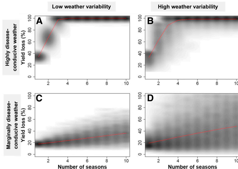
Fig. 2. Long-term (10 season) yield loss under no-management scenarios, with low starting levels of infection, under highly and marginally disease-conductive weather scenarios with high (0.3) and low (0.1) season-to-season variability in weather, in the absence of external inoculum (based on 2,000 simulations). Other parameters are set to default values in Table 2. Red lines indicate the mean value.
