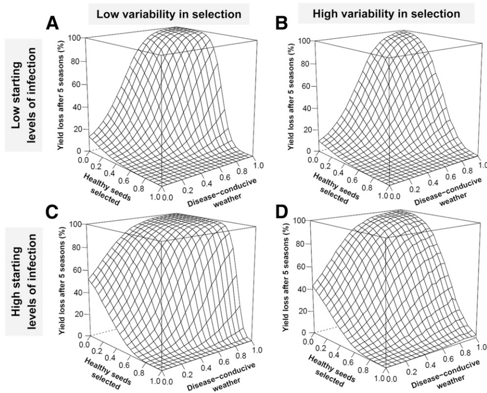
Fig. 5. Percent yield loss after 5 seasons as a function of the mean effectiveness of seed selection (proportion healthy seeds selected) for the range of potential levels of disease-conduciveness of weather, at low (A, B) and high (C, D) starting levels of infection, and low (0.1; A, C) and high (0.3; B, D) variability in selection, in the absence of external inoculum (based on 2,000 simulations). Seed selection is expressed in terms of the effectiveness of implementation. Other parameters were set to the default values in Table 2.
