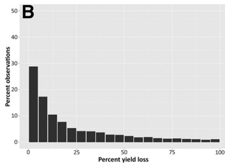
Fig. 6. An illustration of the impact of including expert opinion about the frequency distribution of resistance deployment, compared with an analysis with no information about resistance deployment, for one scenario. A , Mean of experts' estimate of cassava field acreage under different resistance levels. B , Distribution of yield loss in the absence of information on resistance deployment (i.e., all resistance levels are considered equally likely). C , Distribution of yield loss when experts' estimate is used to weight resistance levels. The other parameters used in the illustration are pHS_0 = 0.8 , K = 100 , E = 0 , \beta = 0.02 , W = 0.3 (high variability [0.3]), M = 1 (low variability [0.1]), A = 1 (low variability [0.1]), G = 4 , Z = 1 (low variability [0.1]), Y = 0.9 , R = 0.1 , \phi = 0 , \theta = 0.2 .
