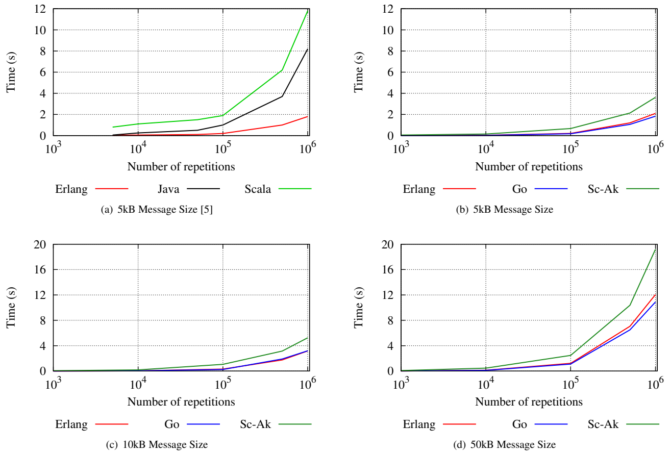
Figure 3. PingPing Benchmark
