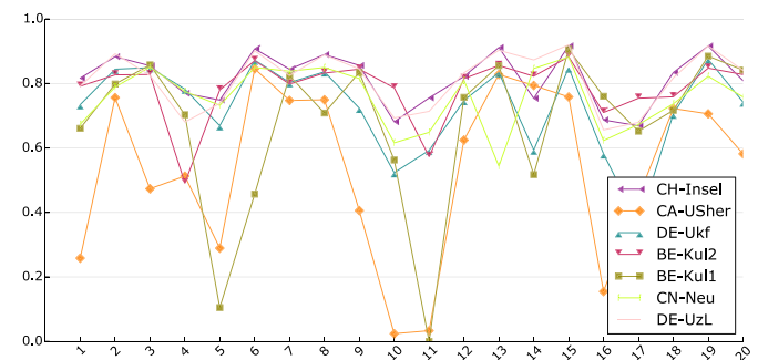
Fig. 9. DC score result of all 7 SPES teams for each of the testing dataset cases. Most methods show a similar pattern. Please refer to the online version for color.
