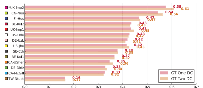
Fig. 5. Differences in performance on the two ground truth sets. The graph shows each methods average DC scores on the 36 testing dataset cases broken down by ground truth set. A star (*) before a team's name denotes statistical significant difference according to a paired Student's t -test with p < 0.05 . The methods are color coded. (For interpretation of the references to colour in this figure legend, the reader is referred to the web version of this article.)
