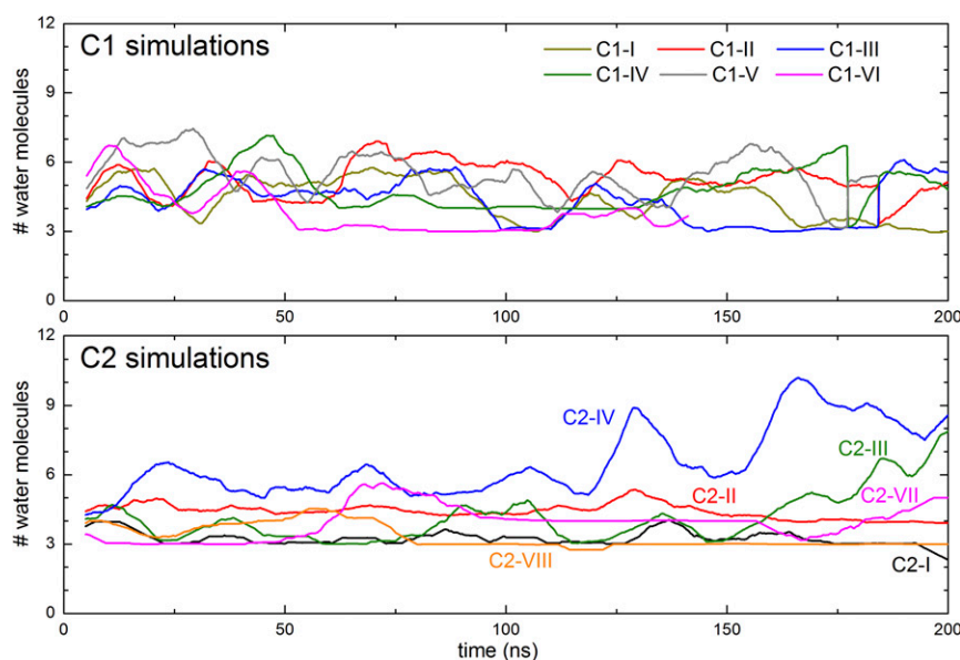
Fig. 2. Time dependencies of numbers of water molecules adjacent to heme a . Only water molecules within 4 Å of the N and O atoms of the side chains of residues 461, 382, 458, 424, 38, 454, 371, 451, 54, and 428 are included. The plot shown is a running average of 100 simulation snapshots taken at 100-ps time intervals.
