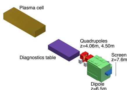
Figure 1: A 3D CAD image of the spectrometer system annotated with distances along the z direction from the exit of the plasma cell to the magnetic centers of magnets, and the center of the scintillator screen.
