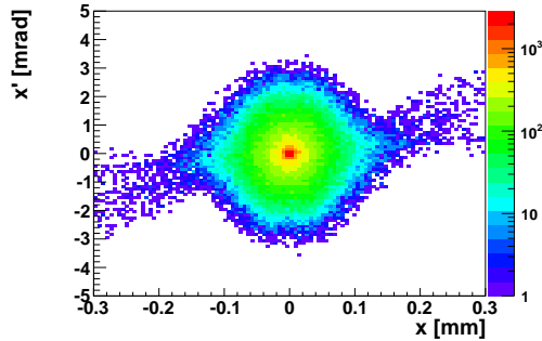
Figure 2: Central region of a sample of the simulated phase space distribution of the witness electron beam.
