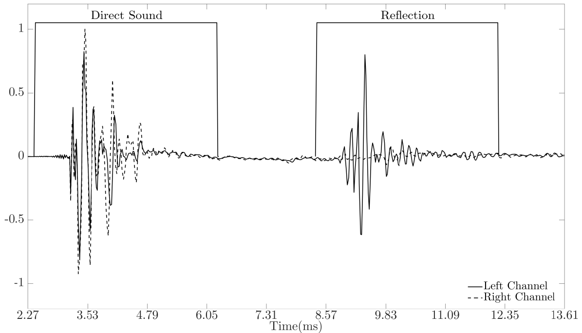
Figure 5. Example binaural room impulse response generated with source at azimuth = 0^\circ and reflector at azimuth = 71^\circ ; the solid line is the left channel of the impulse response; the dotted line is the right channel of the impulse response; and the windowed area denotes the segmented regions using the technique discussed in Section 2.4.
