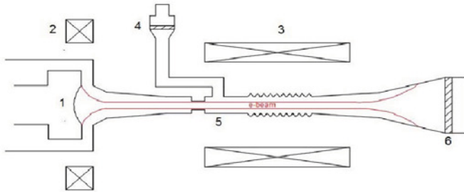
Fig. 1. The schematic of a gyro-TWA. (1) electron gun, (2, 3) coil system, (4) pillbox window, (5) input coupler, (6) output window.
