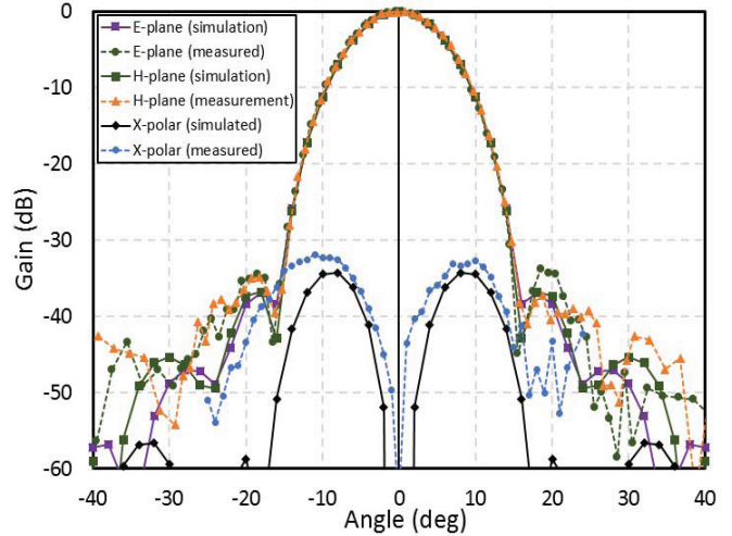
Fig.5 Measured far-field radiation pattern of the broadband W-band gyro-TWA.
