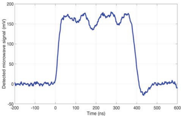
Fig. 4 Measured microwave signal of the broadband W-band gyro-TWA.
