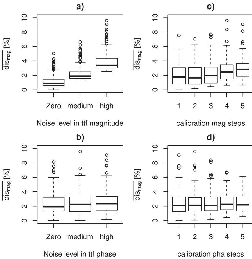
Fig. 10. Quality of calibrated random phase spectra for the four types of departure introduced in the tank transfer function (ttf) and initial calibration function. The four types of departure are explained in section 4.2. Plot a) corresponds to type i, plot b) to type ii, plot c) to type iii and plot d) to type iv. Note: A small number points lying above 10% have been omitted in the illustration.
