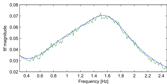
(a) noise level introduced in tank transfer function magnitude
