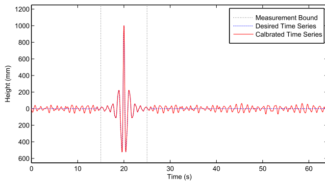
Fig. 2. Water surface elevation time series for the target spectrum and for the converged (calibrated) simulated spectrum.
