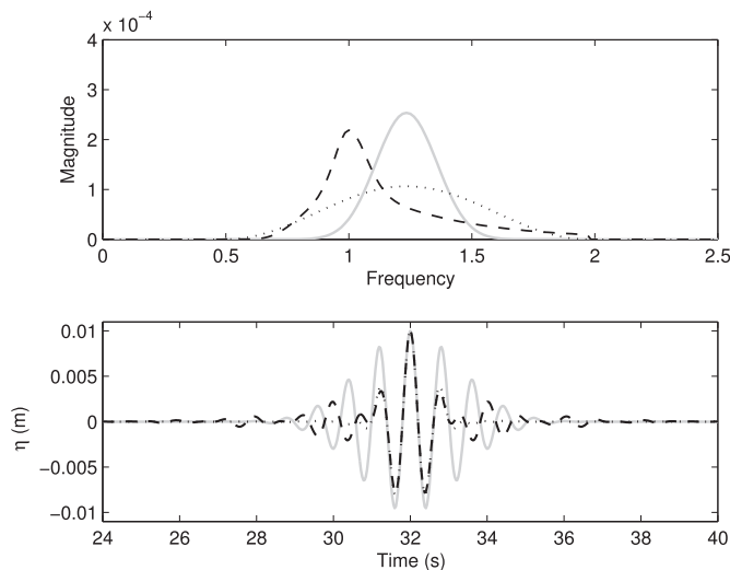
Fig. 5. Comparison of the frequency and the time domain representation of focused wave events based upon: — JONSWAP spectrum, ···· Hanning energy distribution and — DPSS energy distribution.
