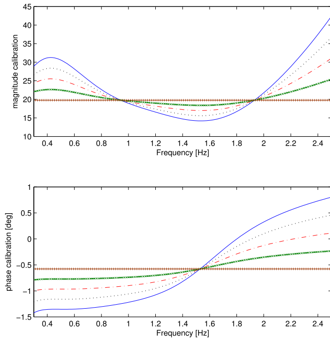
Fig. 7. The initial calibration functions used within the numerical investigation. The constant amplitude/phase calibration functions are referred to as step 1 where the ideal calibration functions are referred to as step 5 .
