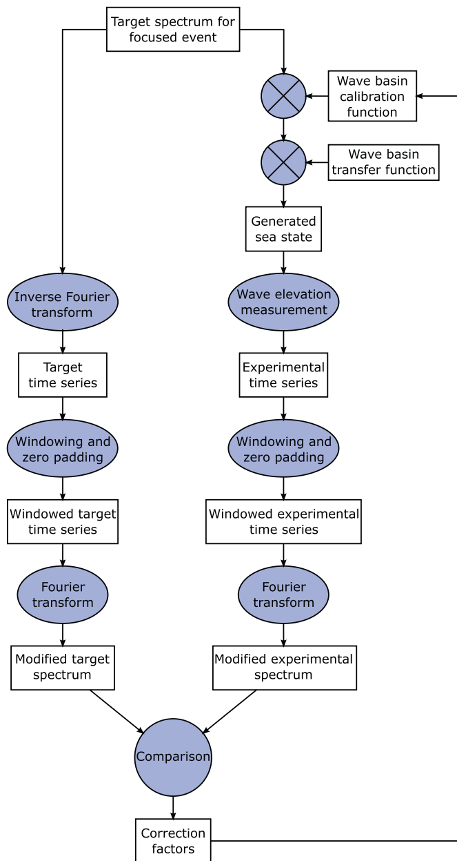
Fig. 1. Iterative focused event calibration process.
