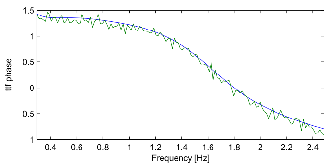
(b) noise level introduced in tank transfer function phase
