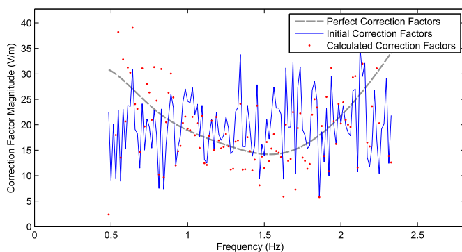
Fig. 4. Magnitude correction factors for the perfect, initial and computed calibrations.
