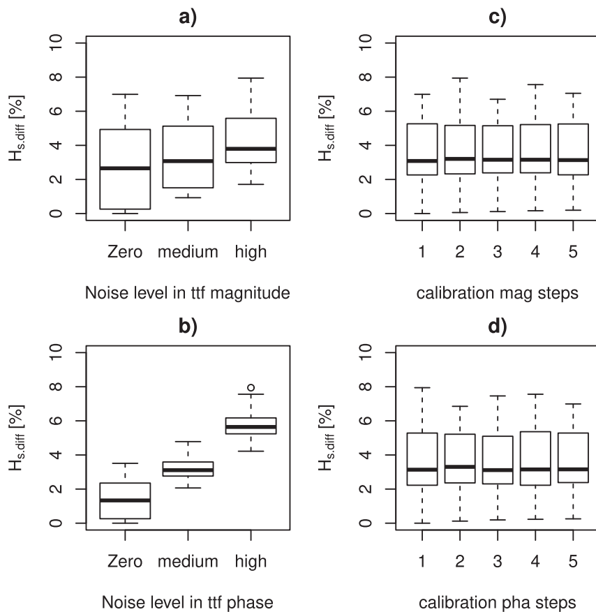
Fig. 11. Quality of the calibrated time series for the four types of departure introduced in the tank transfer function (ttf) and initial calibration function. The four types of departure are explained in section 4.2. Plot a) corresponds to type i, plot b) to type ii, plot c) to type iii and plot d) to type iv.
