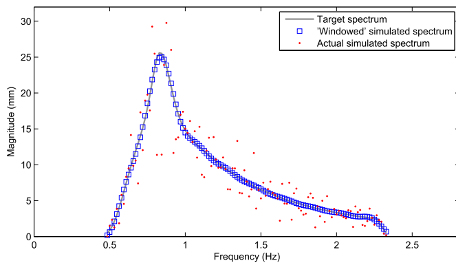
Fig. 3. Comparison of the water surface elevation spectra after calibration, including the spectrum associated with the simulated time series zero-padded outside the measurement window (“Windowed” simulated spectrum), the spectrum computed from the full simulated time series (Actual simulated spectrum) and the target spectrum.
