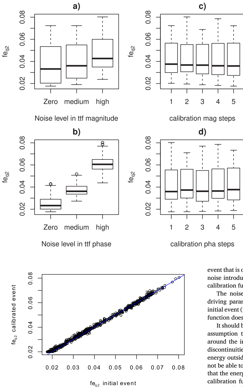
Fig. 9. Quality of the calibrated focused event against the quality of the initial focused event.
