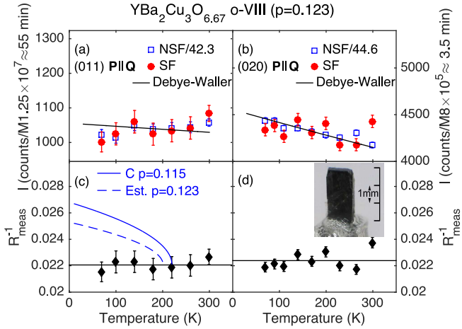
FIG. 9. T -dependence of the scattering for YBCO x = 0.67 . Panels (a-b) show the raw scattering intensity of the SF and NSF channels of the (011) and (020) Bragg reflections. Experimental conditions and data treatment as in Fig. 8. (c-d) The inverse of our measured flipping ratios R_{\text{meas}}^{-1} . The dashed line in (c) shows the expected variation of R_{\text{meas}}^{-1} for a p = 0.123 sample determined by interpolating between samples measured by Fauqué et al. 8,43 (see main text). Solid curve is sample C from the measurements of Fauqué et al. 8 [Fig. 1(a)]. Photo shows the \text{YBa}_2\text{Cu}_3\text{O}_{6.67} single crystal used in this work.
