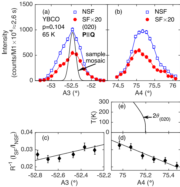
FIG. 6. (a) Rocking curves of a strong, exclusively nuclear Bragg peak (020) as a function of A3 and A4. The FWHM widths are 0.58^\circ and 0.67^\circ respectively. (b) Data in the spin-flip (SF) channel has been multiplied by a factor of 20 for presentation. (c)-(d) Variation of the corresponding inverse flipping ratio R_{\text{inst}}^{-1} over the rocking curve ranges of panes (a)-(b). Data were collected at 65K. The solid line in (a) indicates the sample mosaic profile as measured by 100 keV x-ray diffraction 32 . (e) The T -dependence of the scattering angle 2\theta of the (020) Bragg reflection based on the data of Božin et al. 50 .
