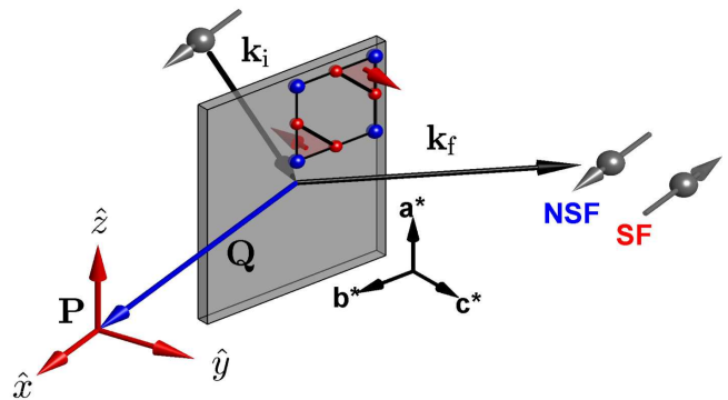
FIG. 3. Longitudinal polarization analysis (LPA) setup used in this experiment. The neutron polarization used was \mathbf{P} \parallel \mathbf{Q} . The initial and final wavevectors of the neutron are labelled by \mathbf{k}_i and \mathbf{k}_f .
