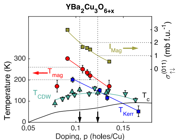
FIG. 2. YBCO phase diagram. (left axis) Superconducting transition temperature, T_c , versus hole doping p (black line). Also included are onset temperatures of CDW order T_{\text{CDW}} ( \blacktriangle , 34 and \blacktriangledown , Ref. 41), putative \mathbf{q} = 0 AFM order T_{\text{mag}} 8,9,42 and the Kerr anomaly T_{\text{Kerr}} 30 . (right axis) Doping dependence of the magnetic intensity at the (011) Bragg reflection reported in Refs. 8, 9, 42, and 43. Doping levels of the x = 0.54 and x = 0.67 samples used in the present study are denoted by the arrows and the horizontal dotted lines indicate corresponding values of T_{\text{mag}} and \sigma_{\uparrow\downarrow}^{(011)}(T \approx T_c) .
