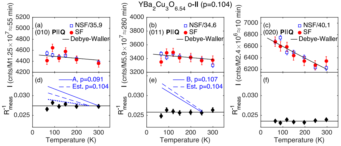
FIG. 8. T -dependence of the scattering for YBCO x = 0.54 . (a)-(c) show the raw SF/NSF scattering intensity of the (010), (011) and (020) Bragg reflections. No background subtractions have been made, the NSF data are scaled by the constants indicated. (d-f) display the inverse flipping ratios R_{\text{meas}}^{-1} determined from the data in (a-c). In this case, a measured T -independent background is subtracted (see main text). Dashed lines in (d) and (e) show the estimated variation of R_{\text{meas}}^{-1} for p = 0.104 determined by interpolating between samples measured by Fauqué et al. 8,43 . Solid lines are samples with the closest doping [i.e. sample A from Fig. 2(b) and sample B from Fig. 1(c) of Ref. 8]. We use Eqn. 8 with \sigma_{\uparrow\uparrow} = |F_N|^2 = 1.84 and 0.28 barn f.u. -1 for (010) and (011) respectively. See main text for more details and dotted line.
