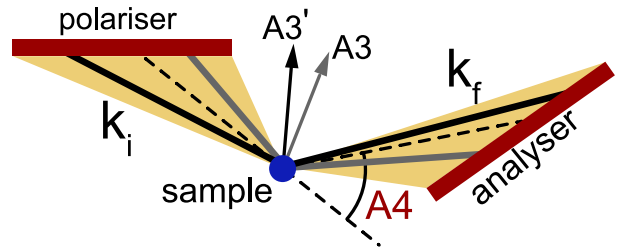
FIG. 5. The small mosaic of the sample means that only part of the monochromator and analyzer crystals are selected. For example, the grey (black) lines show \mathbf{k}_i and \mathbf{k}_f for sample rotation angle A3 (A3'). At each temperature, the sample rotation (A3) and the position of the analyzer (A4) were scanned to select the same part of the monochromator and analyzer. A4 is the scattering angle corresponding to the center of analyzer.
