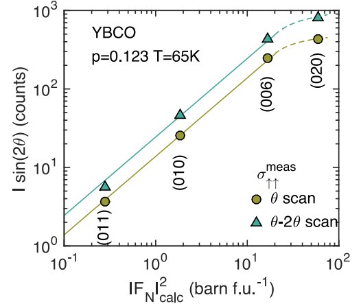
FIG. 10. A comparison of the measured integrated intensity of the nuclear Bragg peaks ( p = 0.123 sample) times Lorentz correction factor with the calculated structure factors ( |F_N|_{\text{calc}}^2 ). The data are collected under the same conditions as the rest of the experiment. The Lorentz factor 39,56,57 corrects for different scattering angles 2\theta . The structure factors are calculated using data in Jorgensen et al. 53 . The solid lines are fits to I \sin(2\theta) \propto |F_N|_{\text{calc}}^2 .
