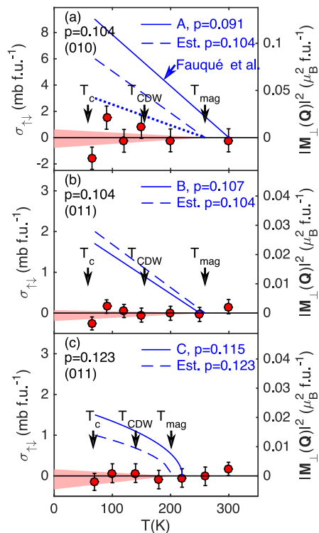
FIG. 11. T -dependence of the magnetic cross section \sigma_{\uparrow\downarrow} and magnetic structure factor squared |\mathbf{M}_{\perp}(\mathbf{G})|^2 determined from R_{\text{meas}}^{-1} in Figs. 8(d-e) and 9(c). Eqs. 8 and 9 are used to carry out conversions with |F_N|^2 = 1.85, 0.28 \text{ barn f.u.}^{-1} for \mathbf{G} = (010) and (011) . Filled pink region shows the one standard deviation range of linear fits to the data. Arrows show onset temperatures for superconductivity (Table II), T_c , 2-D charge density wave order 32,33 , T_{\text{CDW}} and putative orbital ordering 8 , T_{\text{mag}} . The meanings of the solid, dashed and dotted lines is explained in the main text and captions to Figs. 8 and 9.
