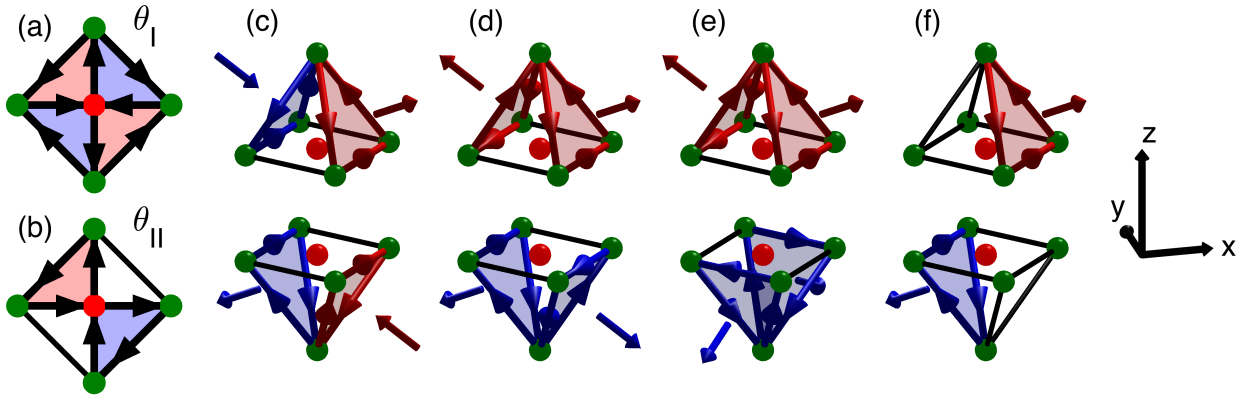
FIG. 1. Some possible configurations of the CC-order in \text{YBa}_2\text{Cu}_3\text{O}_{6+x} . Panels (a,b) show the original \text{CC-}\theta_I and \text{CC-}\theta_{II} states proposed by Varma 6 in which current flows within the \text{CuO}_2 planes. (c)-(f) Show arrangements based on those proposed by Yakovenko 18,19 in which current flows out of the \text{CuO}_2 planes. The oxygen pyramids which make up the bilayer structure are shown with copper ions as red spheres and oxygen ions as green. Arrows connecting ions indicate the direction of orbital current flow. Arrows outside the unit cell indicate the resulting moments and are colored red for those with a component along the z -axis and blue for those with one along -z .
