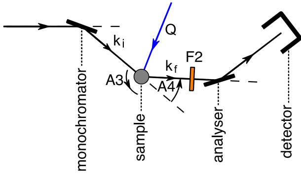
FIG. 4. Schematic of the IN20 spectrometer in the horizontal plane. Neutrons are monochromated and polarized using Heusler-alloy monochromator. The neutron spin-state is maintained using a small guide field throughout the spectrometer. The Heusler analyzer scatters spin of one polarization to the detector. A Mezei coil flipper 36 F2 can be switched on to flip the polarization of neutrons. This determines which polarization the analyzer system detects.
