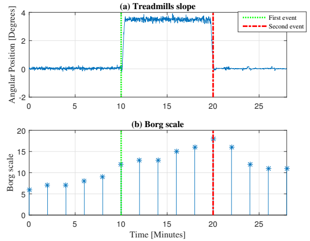
Fig. 7. The physical activity difficulty parameters: (a) Treadmill inclination angle recorded using the MPU9150 IMU sensor and (b) Patient's fatigue obtained from the user interface.
