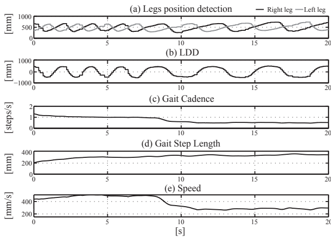
Fig. 3. Experiment with speed variation from 500 to 250 mm/s. (a) Legs' position detection from the LRF. (b) Legs Difference Distance(LDD). (c) GC estimation. (d) Step length estimation. (e) Human linear velocity.
