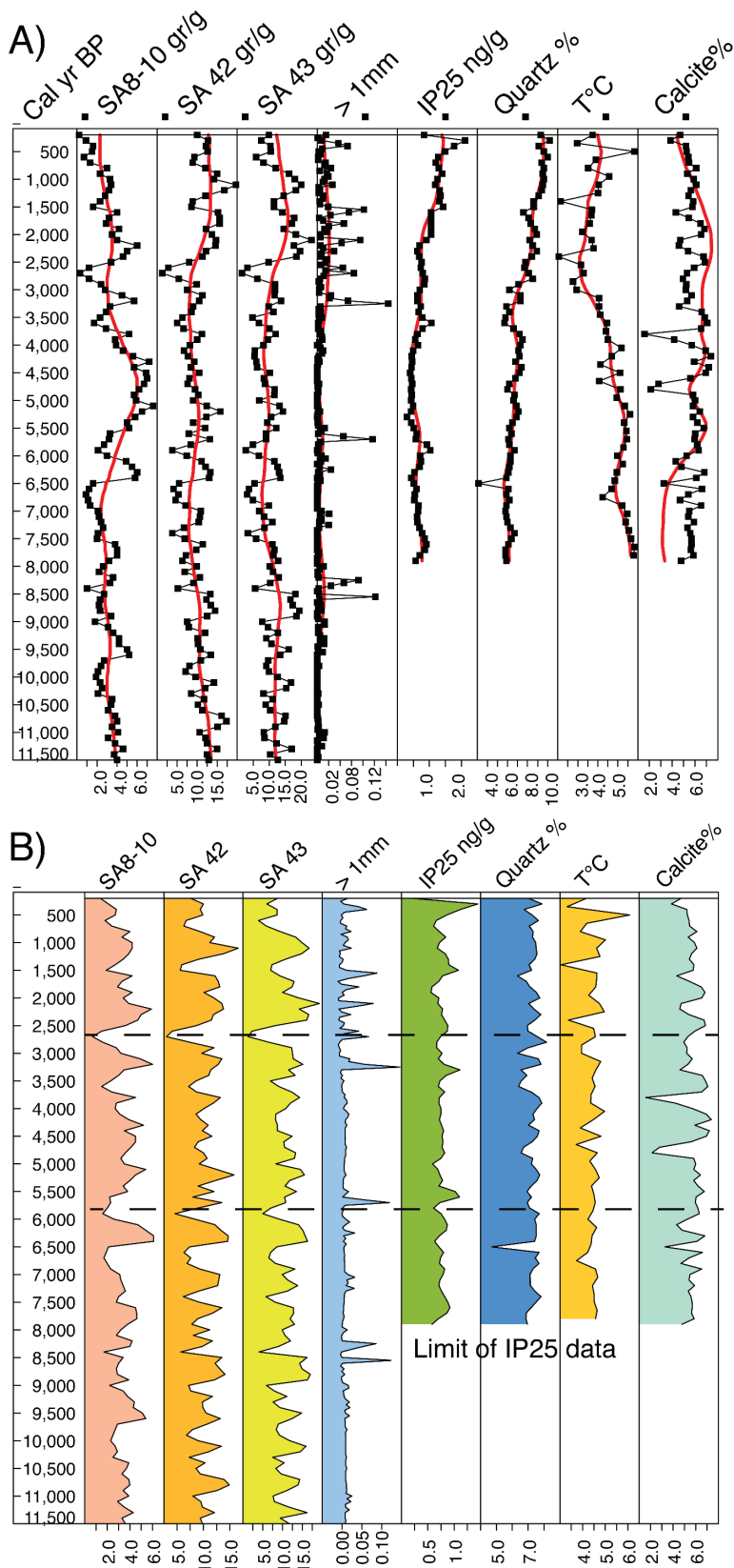
FIGURE 4. (A) Trends and integrated, equispaced data of the 100-yr equitime series of environmental parameters compared to those in the Fe grain matches to important source areas and IP_{25} values for core 2322. The Western Canadian Arctic (WCA), represents SA8-10 (Fig. 1). Red lines show the trends in the data, black lines are the original data. (B) Color panels show the detrended data (Table 1). Where no trend was detected (e.g., SA43) we plotted the reconstructed signal from the 1st SSA/PCA scores.
