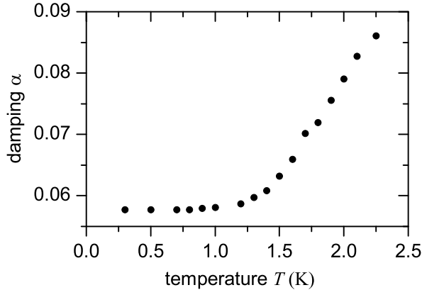
FIG. 4. Plot of \alpha(T) obtained by means of fitting IVCs as described in the text.
