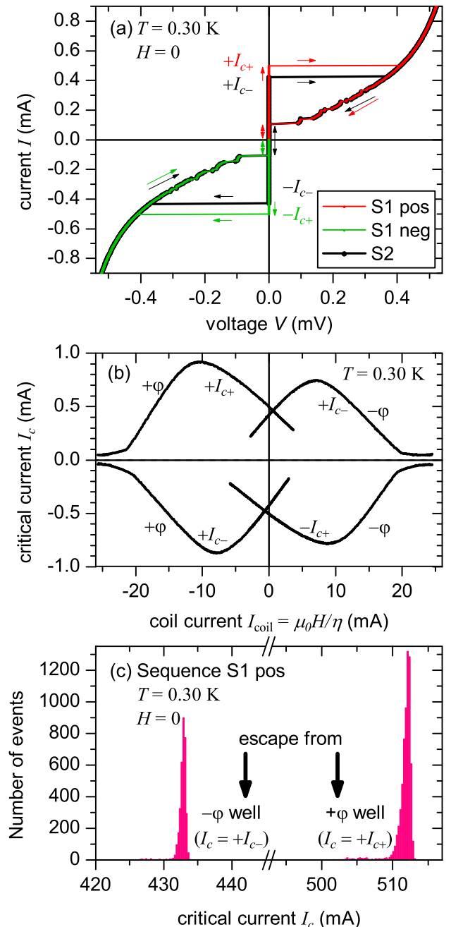
FIG. 2. (Color online) Current-voltage characteristic (a), critical current dependence on the magnetic field (b) and escape histogram (c) at T = 0.30 K. In (a), different colors correspond to different sweep sequences of the bias current I . In (b), the magnetic field is applied in-plane of the junction by means of a coil with \mu_0 H = \eta \cdot I_{\text{coil}} with the coil factor \eta \sim 5 \mu\text{T}/\text{mA} . The histogram in (c), measured by using sequence S1 pos, shows two peaks corresponding to the two critical currents I_{c\pm} .
