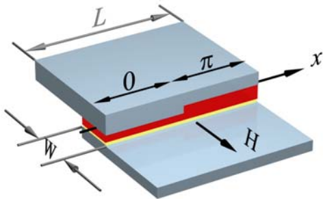
FIG. 1. Sketch of the sample under investigation — a (from bottom to top) Nb|AlO|CuNi|Nb JJ of length L \sim \lambda_J and width w \ll L . The critical temperature of the device T_c \sim 9 K. The magnetic field H is applied along y direction, see the figure.
