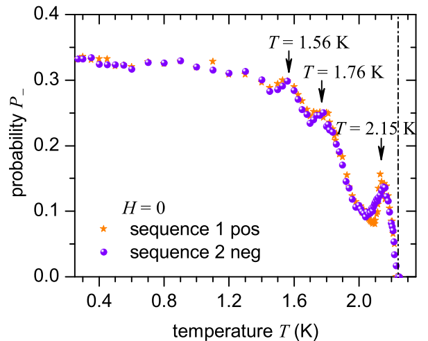
FIG. 3. (Color online) Retrapping probability P_- of the phase in the -\varphi of the Josephson potential U(\psi) for different temperatures T at zero applied magnetic field H . The two set of data correspond to two different sweep sequence of the bias current I .
