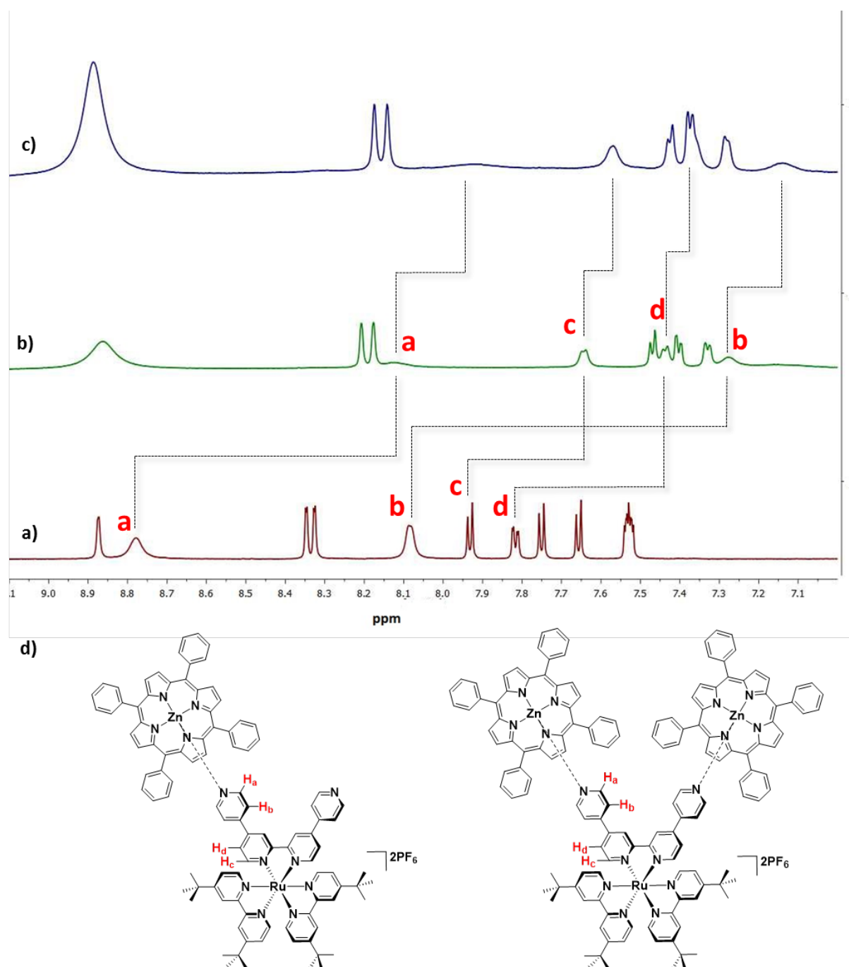
Figure 2. ^1\text{H} NMR spectra in \text{CD}_2\text{Cl}_2 , 500 MHz at 298 K. The concentration of 1 was kept constant at 3.06 mM. a) ^1\text{H} NMR spectrum of 1 ; b) ^1\text{H} NMR spectrum of the assembly 1a ,
