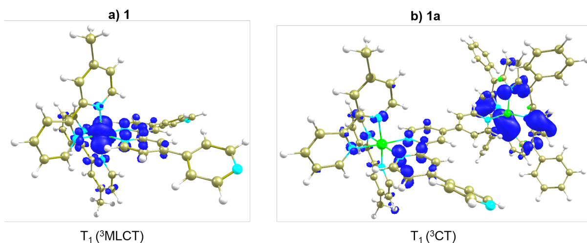
Figure 6. Spin-density distributions [B3LYP/6-31G(d) – ecp-28-mwb for Ru] at the optimized geometry of the lowest triplet excited state of 1 (a) and 1a (b).
