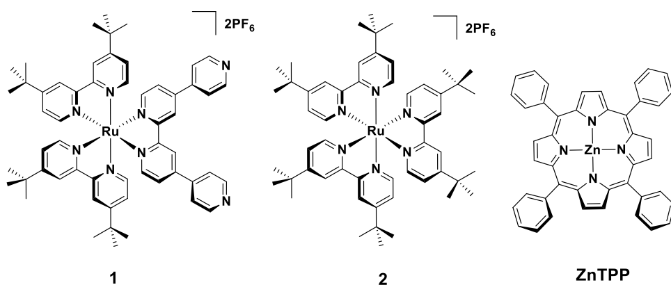
Chart 1. Chemical structures of the reference mononuclear Ru(II) complexes 1 and 2 and ZnTPP under investigation in this work.
