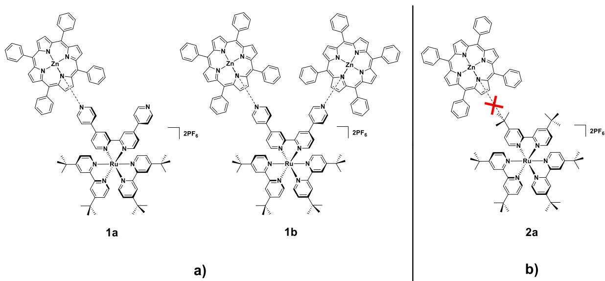
Chart 1. Chemical structures of the reference mononuclear Ru(II) complexes 1 and 2 and ZnTPP under investigation in this work.
