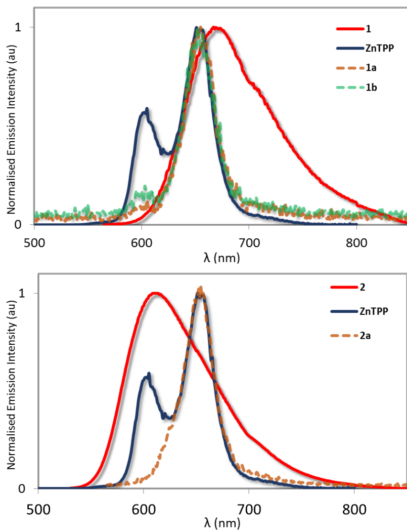
Figure 7. a) Normalized luminescence spectra of 1 (solid red line), ZnTPP (solid blue line), 1a (dotted orange line) and 1b (dotted green line) recorded in degassed DCM at 298 K ( \lambda_{\text{ex}} = 555 nm) with a concentration in the order of 3 \times 10^{-4} M. b) Normalized luminescence spectra of 2 (solid red line), ZnTPP (solid blue line) and of the “non-assembly” 2a (dotted orange line) recorded in degassed DCM at 298 K ( \lambda_{\text{ex}} = 555 nm) with a concentration in the order of 10^{-4} M.
