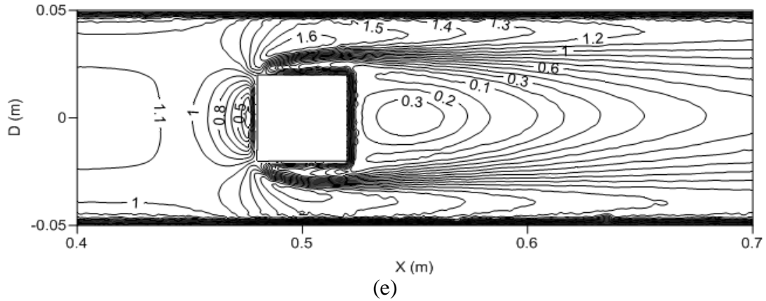
(e) Figure 7 Flow velocity magnitude variations (in m/sec) within a horizontal HCP for the flow of a single equi-density capsule (a) \phi=1 (b) \phi=1.004 (c) \phi=1.02 (d) \phi=2.289 (e) \phi=2.481 of k=0.5 at V_{av}=1 m/sec
