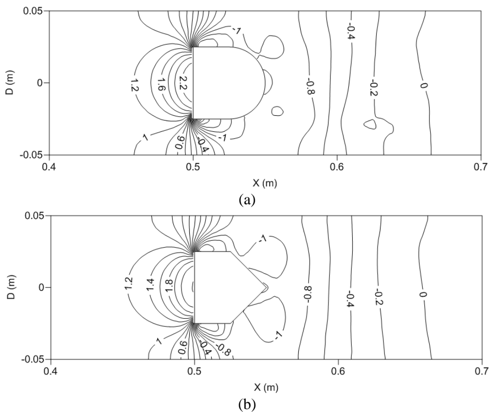
Figure 14 Pressure coefficient variations within a horizontal HCP for the flow of a single equi-density capsule of (a) \phi=1.304 (b) \phi=1.395 of k=0.5 at V_{av}=1 m/sec
