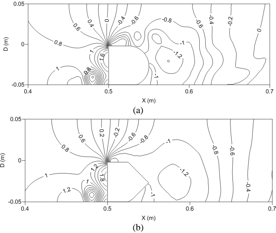
Figure 15 Pressure coefficient variations within a horizontal HCP for the flow of a single heavy-density capsule of (a) \phi=1.304 (b) \phi=1.395 of k=0.5 at V_{av}=1 m/sec
